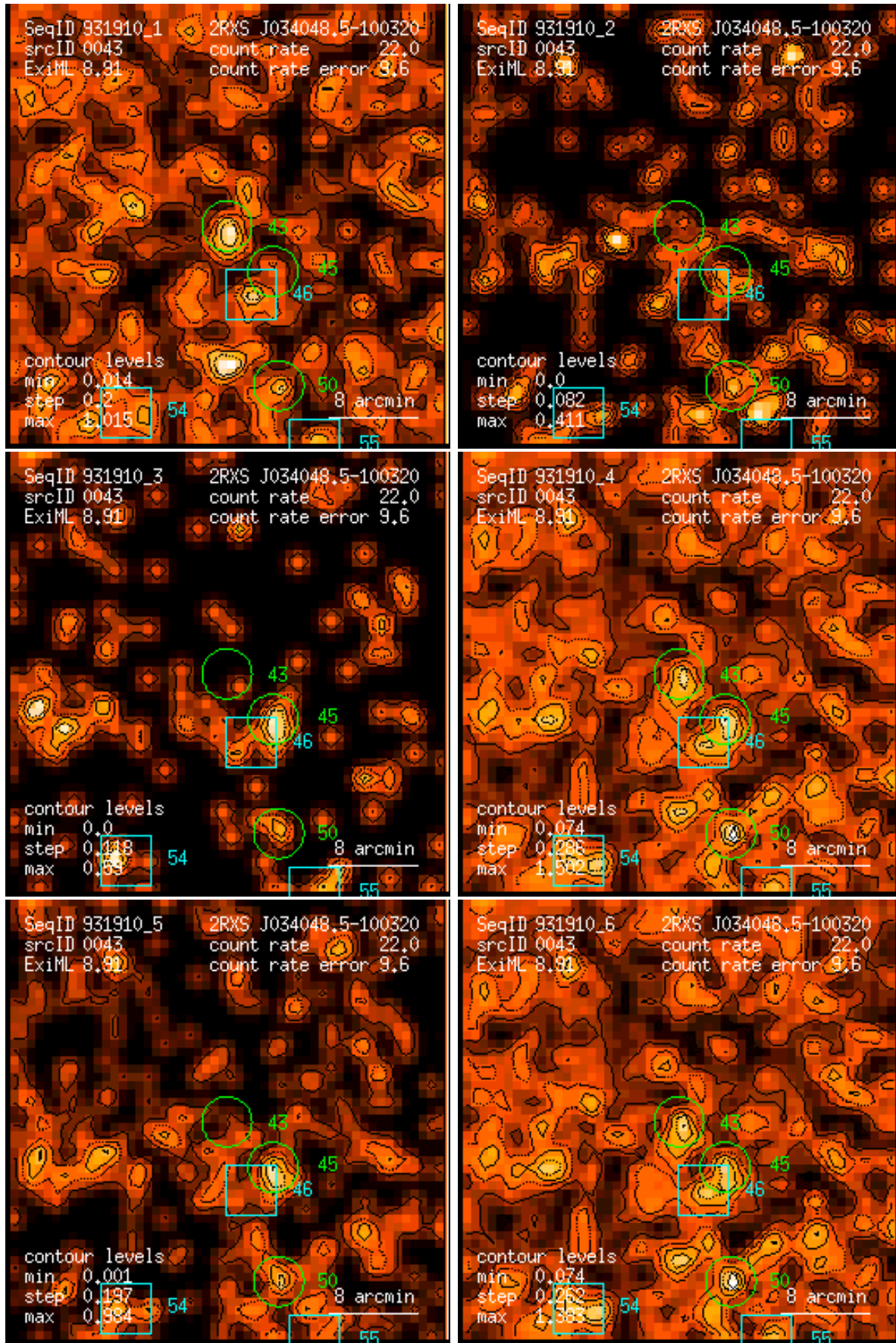
Figure 43: RASS 931910: detection 0043: band rate images, Gaussian filter: (1) PSPC channels 11 – 41, (2) 52 – 90, (3) 91 – 201, (4) 11 – 235, (5) 52 – 201, (6) 11 – 201. Broad band rates in counts/ks. Band rate contour levels in counts/ks/arcmin 2 .
