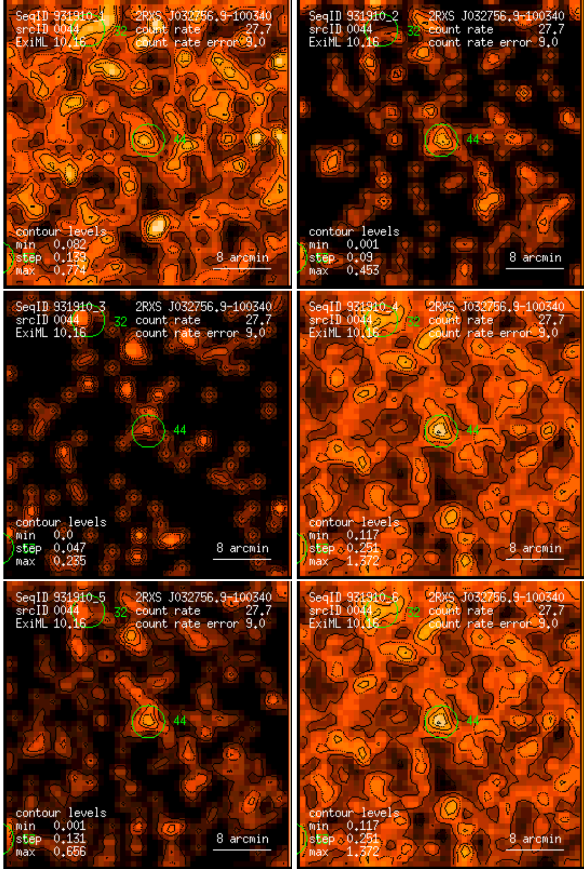
Figure 44: RASS 931910: detection 0044: band rate images, Gaussian filter: (1) PSPC channels 11 – 41, (2) 52 – 90, (3) 91 – 201, (4) 11 – 235, (5) 52 – 201, (6) 11 – 201. Broad band rates in counts/ks. Band rate contour levels in counts/ks/arcmin 2 .
