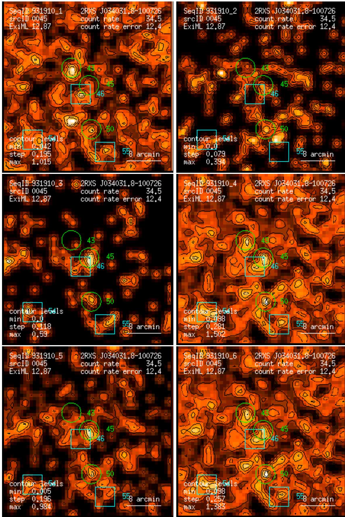
Figure 45: RASS 931910: detection 0045: band rate images, Gaussian filter: (1) PSPC channels 11 – 41, (2) 52 – 90, (3) 91 – 201, (4) 11 – 235, (5) 52 – 201, (6) 11 – 201. Broad band rates in counts/ks. Band rate contour levels in counts/ks/arcmin 2 .
