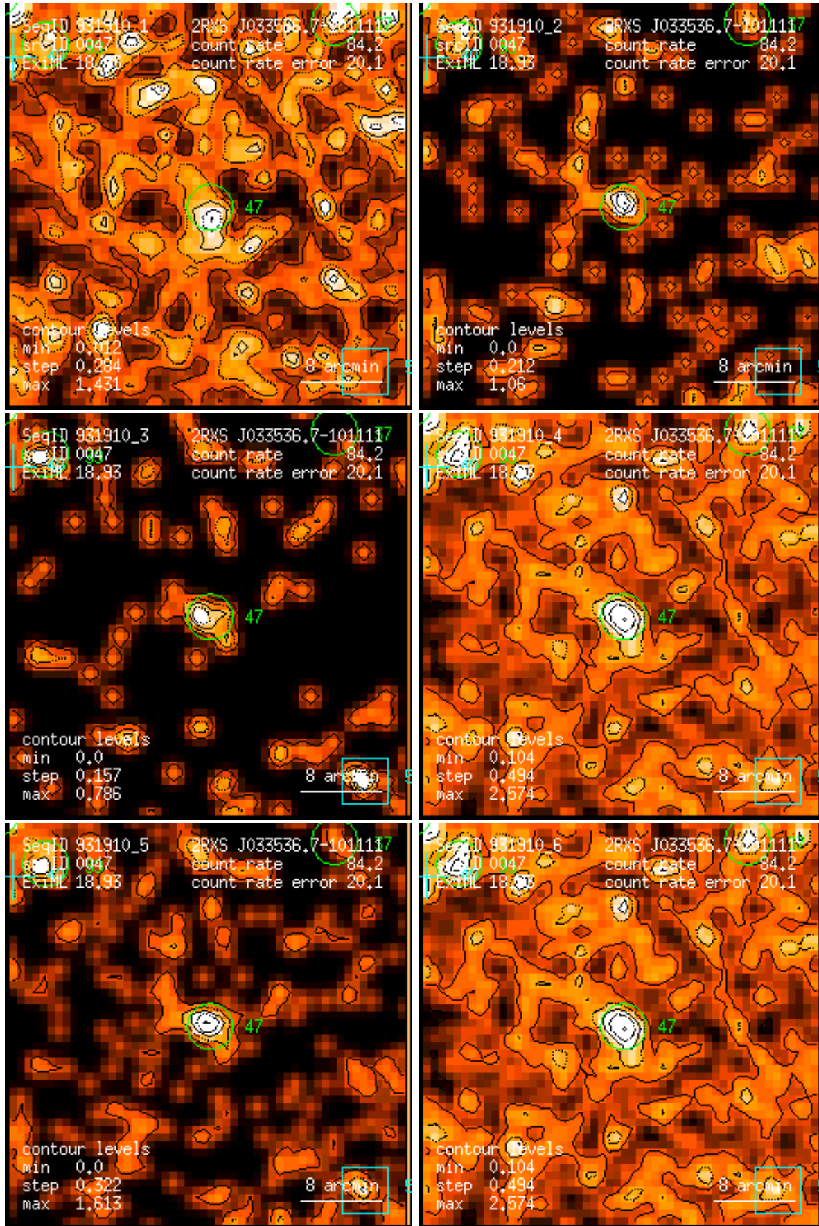
Figure 47: RASS 931910: detection 0047: band rate images, Gaussian filter: (1) PSPC channels 11 – 41, (2) 52 – 90, (3) 91 – 201, (4) 11 – 235, (5) 52 – 201, (6) 11 – 201. Broad band rates in counts/ks. Band rate contour levels in counts/ks/arcmin 2 .
