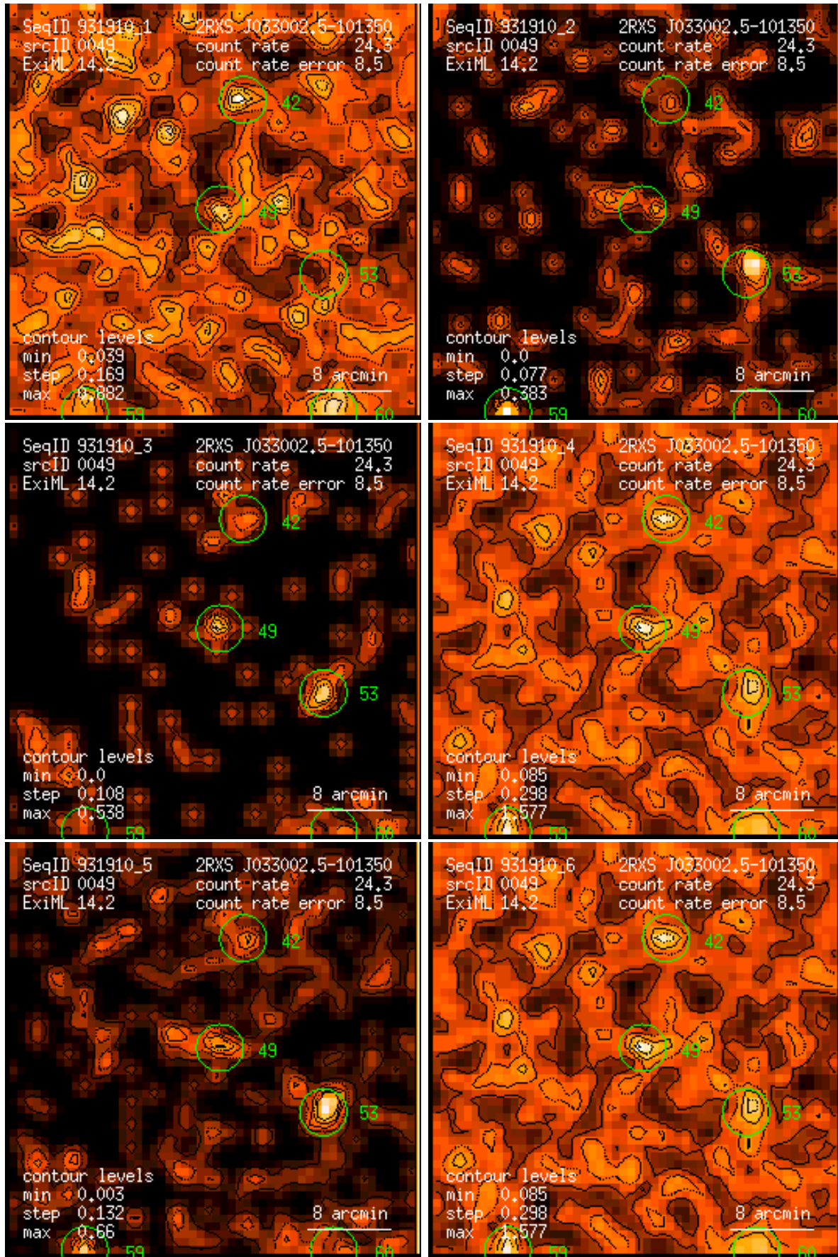
Figure 49: RASS 931910: detection 0049: band rate images, Gaussian filter: (1) PSPC channels 11 – 41, (2) 52 – 90, (3) 91 – 201, (4) 11 – 235, (5) 52 – 201, (6) 11 – 201. Broad band rates in counts/ks. Band rate contour levels in counts/ks/arcmin 2 .
