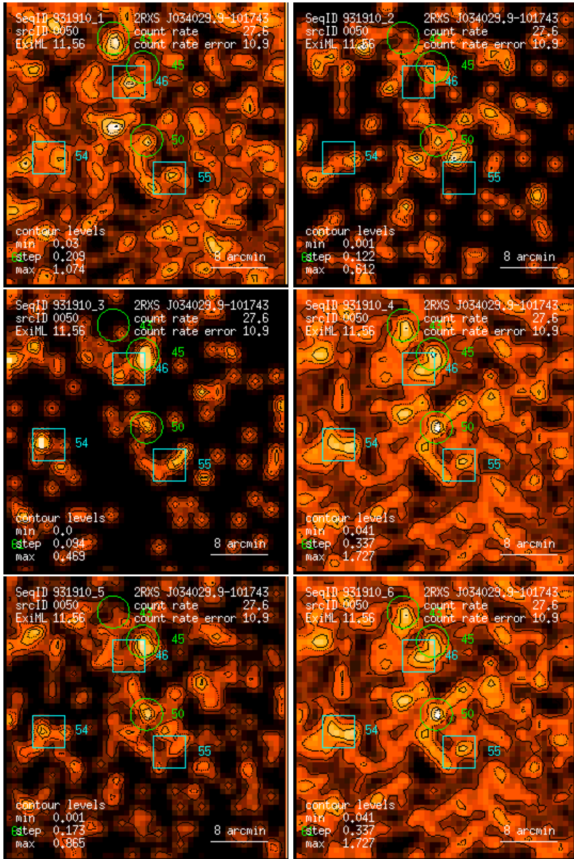
Figure 50: RASS 931910: detection 0050: band rate images, Gaussian filter: (1) PSPC channels 11 – 41, (2) 52 – 90, (3) 91 – 201, (4) 11 – 235, (5) 52 – 201, (6) 11 – 201. Broad band rates in counts/ks. Band rate contour levels in counts/ks/arcmin 2 .
