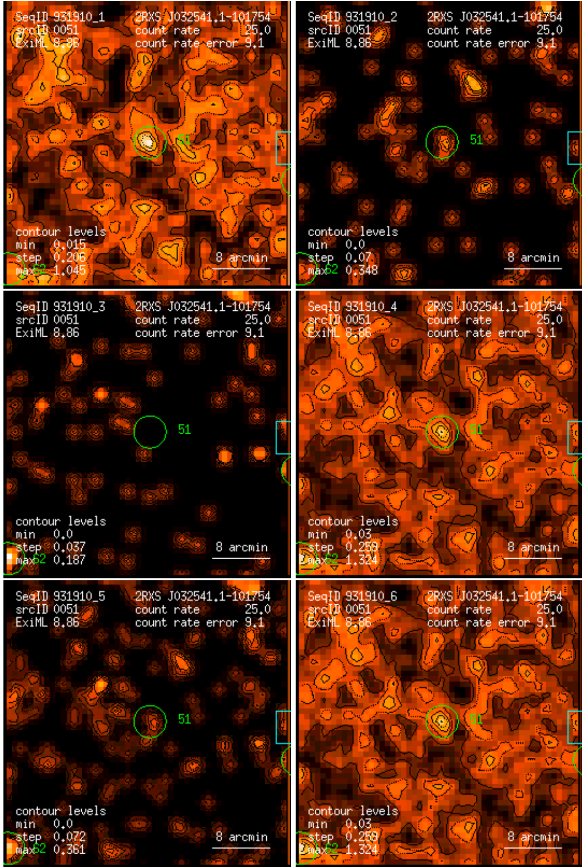
Figure 51: RASS 931910: detection 0051: band rate images, Gaussian filter: (1) PSPC channels 11 – 41, (2) 52 – 90, (3) 91 – 201, (4) 11 – 235, (5) 52 – 201, (6) 11 – 201. Broad band rates in counts/ks. Band rate contour levels in counts/ks/arcmin 2 .
