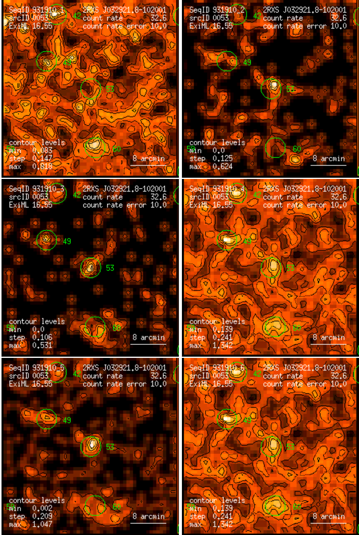
Figure 53: RASS 931910: detection 0053: band rate images, Gaussian filter: (1) PSPC channels 11 – 41, (2) 52 – 90, (3) 91 – 201, (4) 11 – 235, (5) 52 – 201, (6) 11 – 201. Broad band rates in counts/ks. Band rate contour levels in counts/ks/arcmin 2 .
