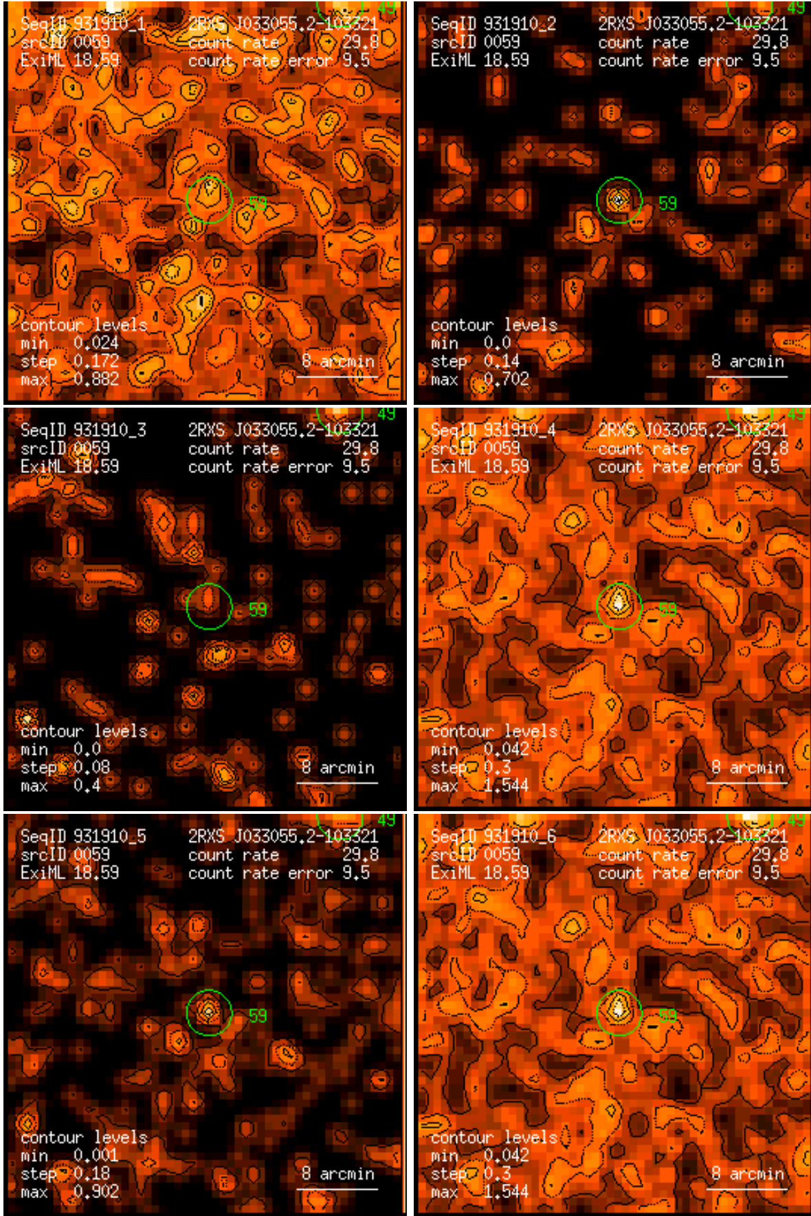
Figure 59: RASS 931910: detection 0059: band rate images, Gaussian filter: (1) PSPC channels 11 – 41, (2) 52 – 90, (3) 91 – 201, (4) 11 – 235, (5) 52 – 201, (6) 11 – 201. Broad band rates in counts/ks. Band rate contour levels in counts/ks/arcmin 2 .
