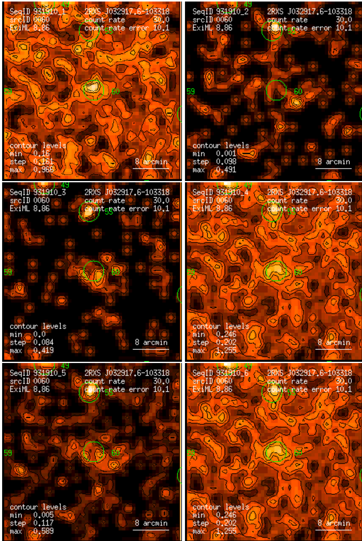
Figure 60: RASS 931910: detection 0060: band rate images, Gaussian filter: (1) PSPC channels 11 – 41, (2) 52 – 90, (3) 91 – 201, (4) 11 – 235, (5) 52 – 201, (6) 11 – 201. Broad band rates in counts/ks. Band rate contour levels in counts/ks/arcmin 2 .
