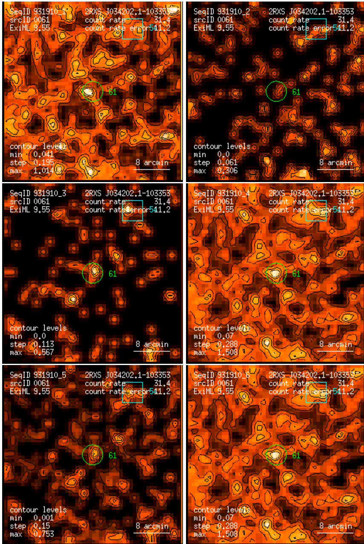
Figure 61: RASS 931910: detection 0061: band rate images, Gaussian filter: (1) PSPC channels 11 – 41, (2) 52 – 90, (3) 91 – 201, (4) 11 – 235, (5) 52 – 201, (6) 11 – 201. Broad band rates in counts/ks. Band rate contour levels in counts/ks/arcmin 2 .
