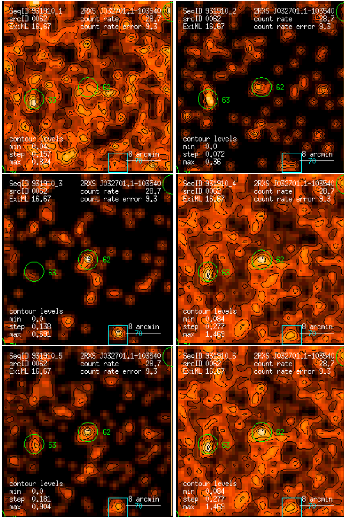
Figure 62: RASS 931910: detection 0062: band rate images, Gaussian filter: (1) PSPC channels 11 – 41, (2) 52 – 90, (3) 91 – 201, (4) 11 – 235, (5) 52 – 201, (6) 11 – 201. Broad band rates in counts/ks. Band rate contour levels in counts/ks/arcmin 2 .
