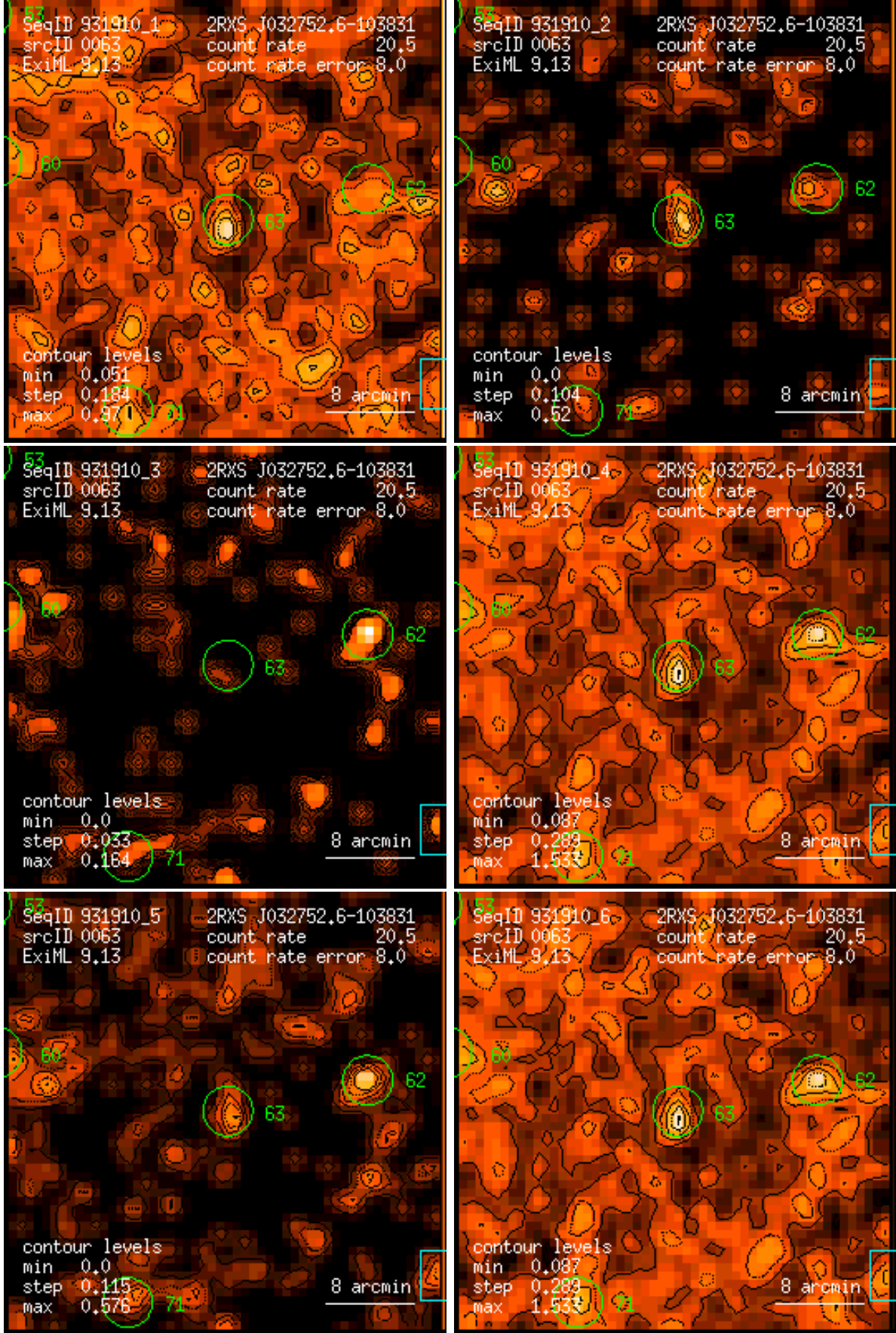
Figure 63: RASS 931910: detection 0063: band rate images, Gaussian filter: (1) PSPC channels 11 – 41, (2) 52 – 90, (3) 91 – 201, (4) 11 – 235, (5) 52 – 201, (6) 11 – 201. Broad band rates in counts/ks. Band rate contour levels in counts/ks/arcmin 2 .
