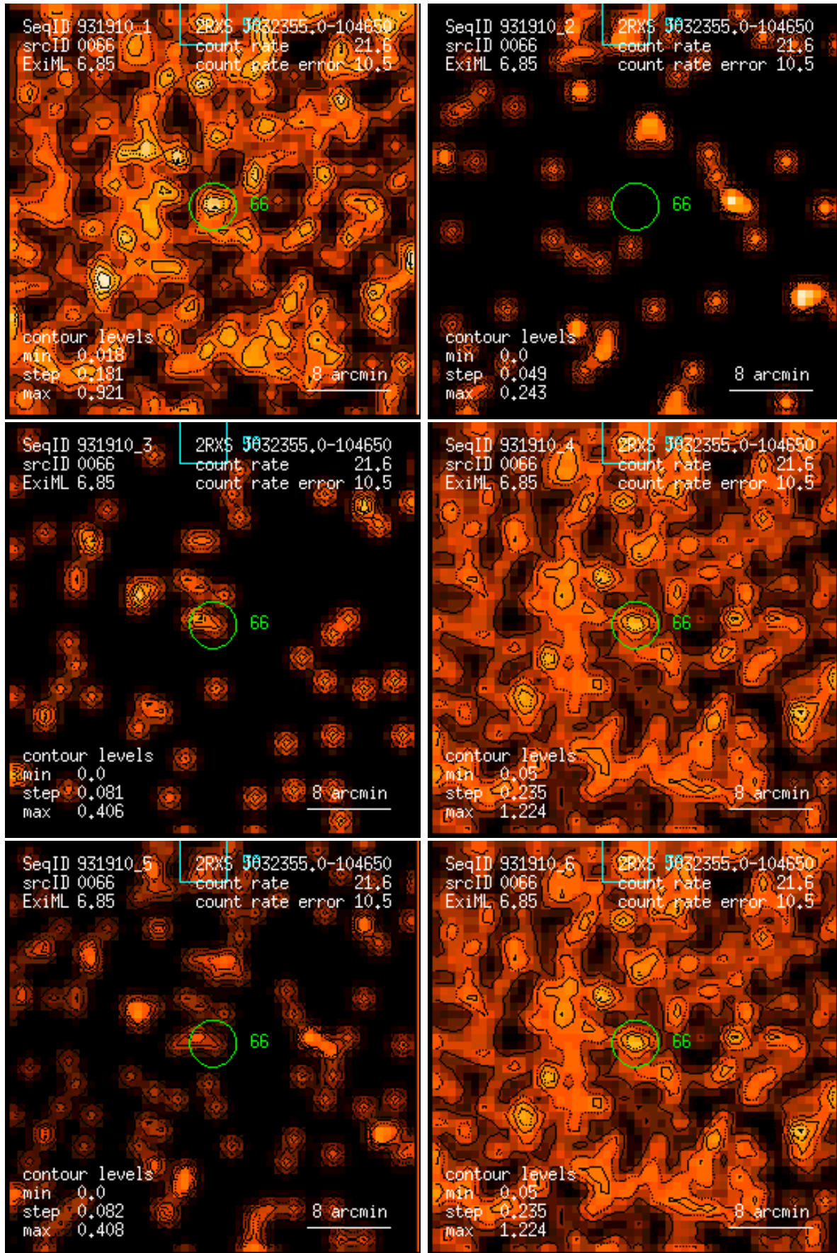
Figure 66: RASS 931910: detection 0066: band rate images, Gaussian filter: (1) PSPC channels 11 – 41, (2) 52 – 90, (3) 91 – 201, (4) 11 – 235, (5) 52 – 201, (6) 11 – 201. Broad band rates in counts/ks. Band rate contour levels in counts/ks/arcmin 2 .
