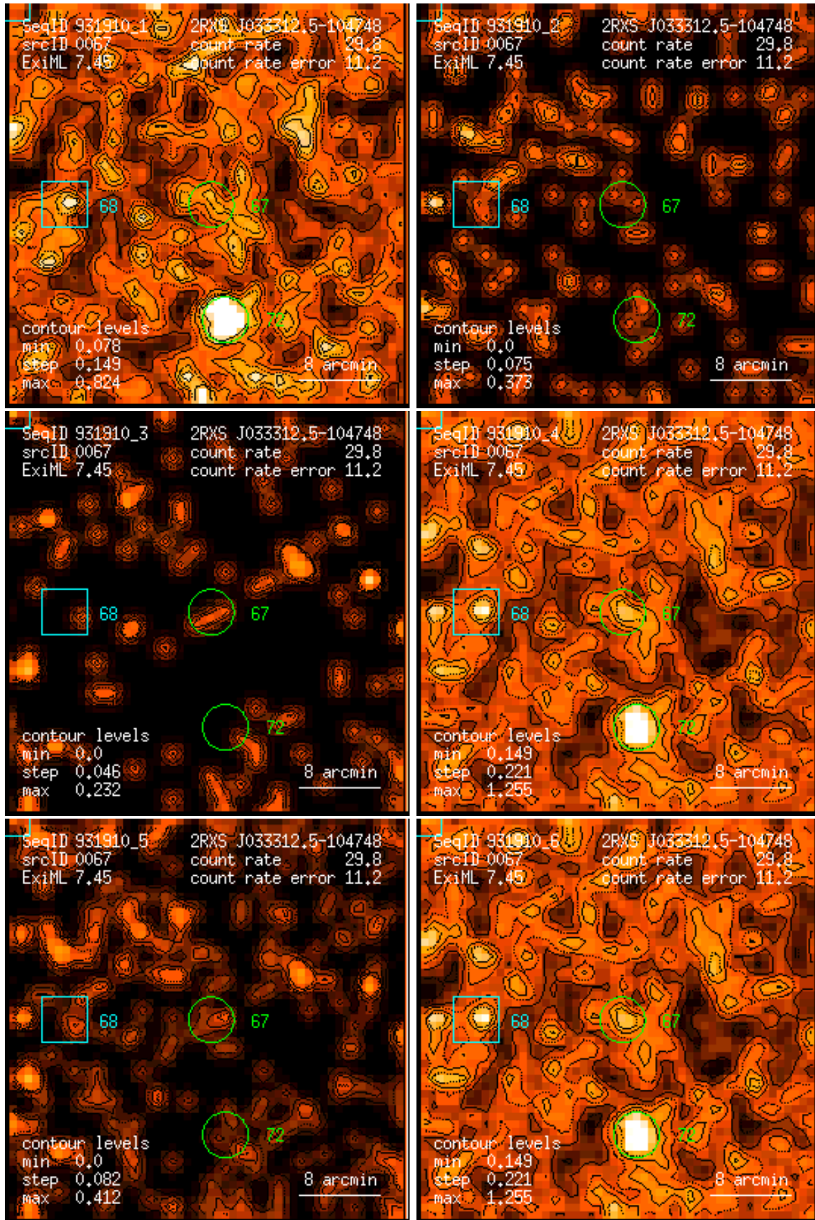
Figure 67: RASS 931910: detection 0067: band rate images, Gaussian filter: (1) PSPC channels 11 – 41, (2) 52 – 90, (3) 91 – 201, (4) 11 – 235, (5) 52 – 201, (6) 11 – 201. Broad band rates in counts/ks. Band rate contour levels in counts/ks/arcmin 2 .
