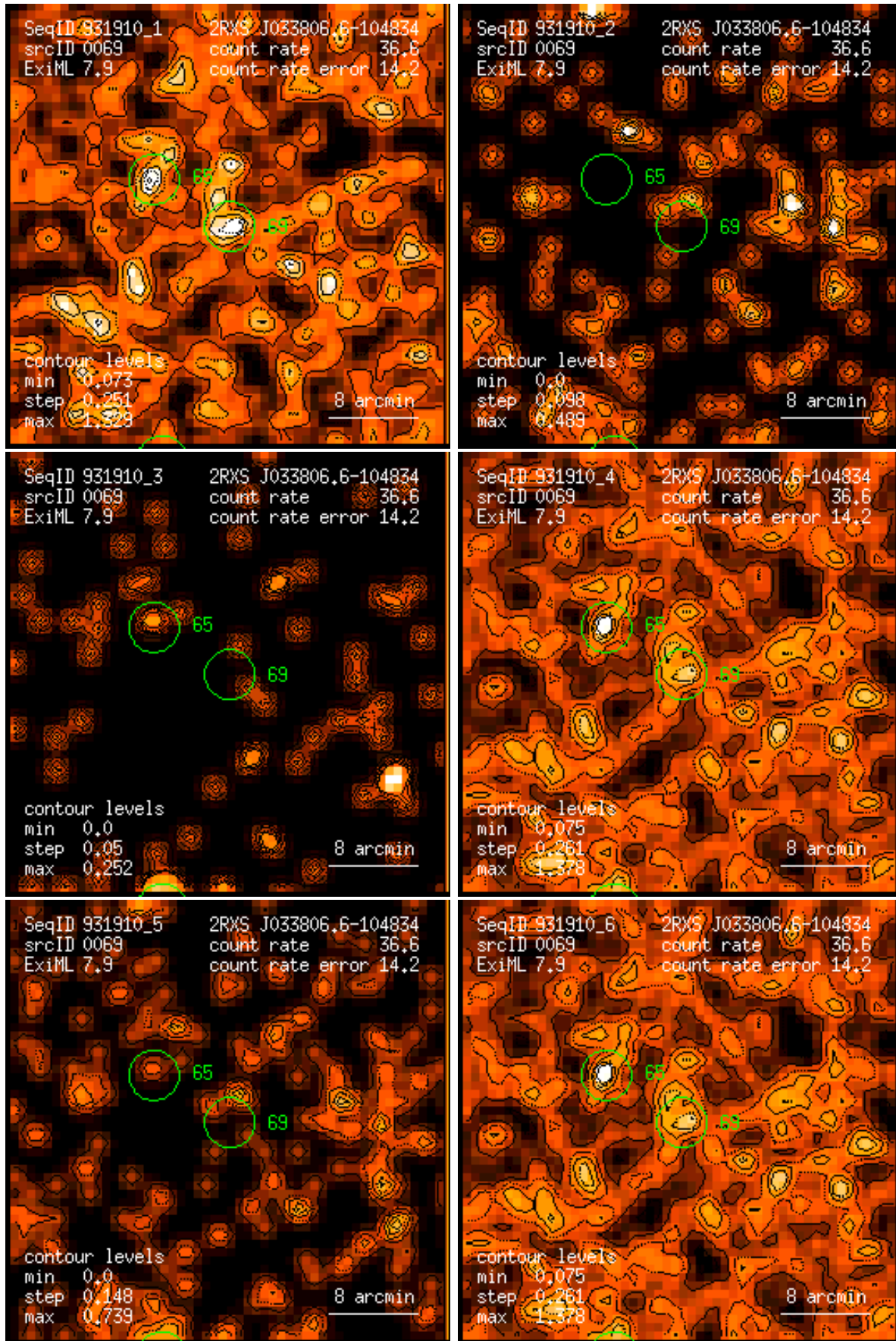
Figure 69: RASS 931910: detection 0069: band rate images, Gaussian filter: (1) PSPC channels 11 – 41, (2) 52 – 90, (3) 91 – 201, (4) 11 – 235, (5) 52 – 201, (6) 11 – 201. Broad band rates in counts/ks. Band rate contour levels in counts/ks/arcmin 2 .
