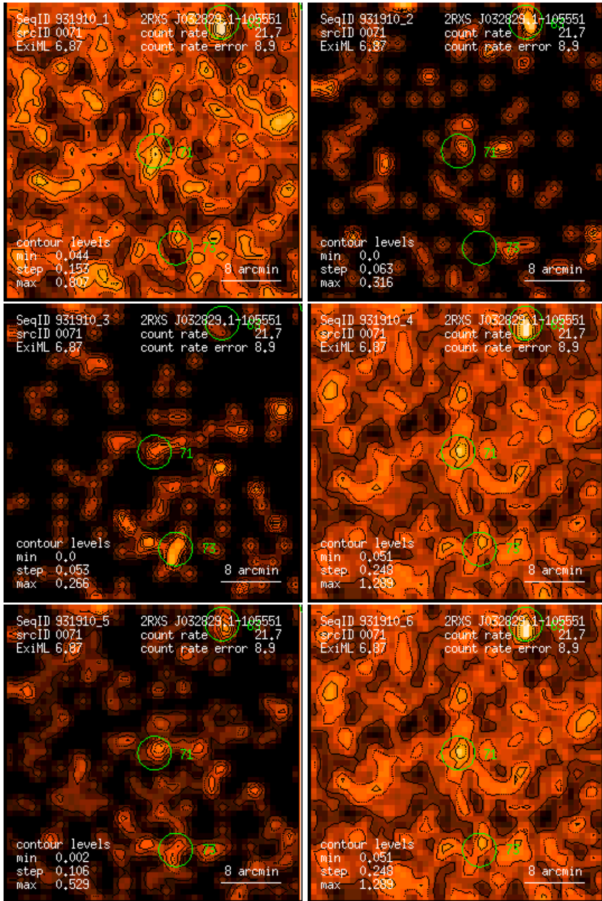
Figure 71: RASS 931910: detection 0071: band rate images, Gaussian filter: (1) PSPC channels 11 – 41, (2) 52 – 90, (3) 91 – 201, (4) 11 – 235, (5) 52 – 201, (6) 11 – 201. Broad band rates in counts/ks. Band rate contour levels in counts/ks/arcmin 2 .
