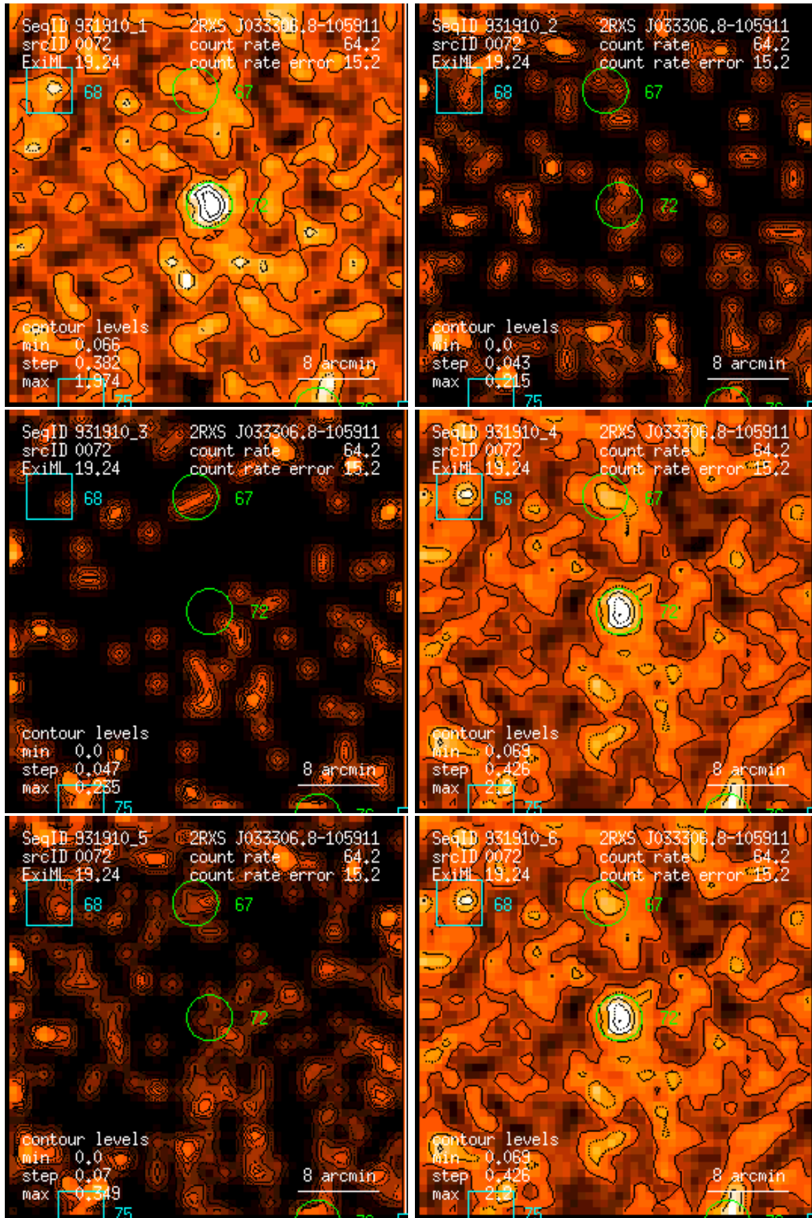
Figure 72: RASS 931910: detection 0072: band rate images, Gaussian filter: (1) PSPC channels 11 – 41, (2) 52 – 90, (3) 91 – 201, (4) 11 – 235, (5) 52 – 201, (6) 11 – 201. Broad band rates in counts/ks. Band rate contour levels in counts/ks/arcmin 2 .
