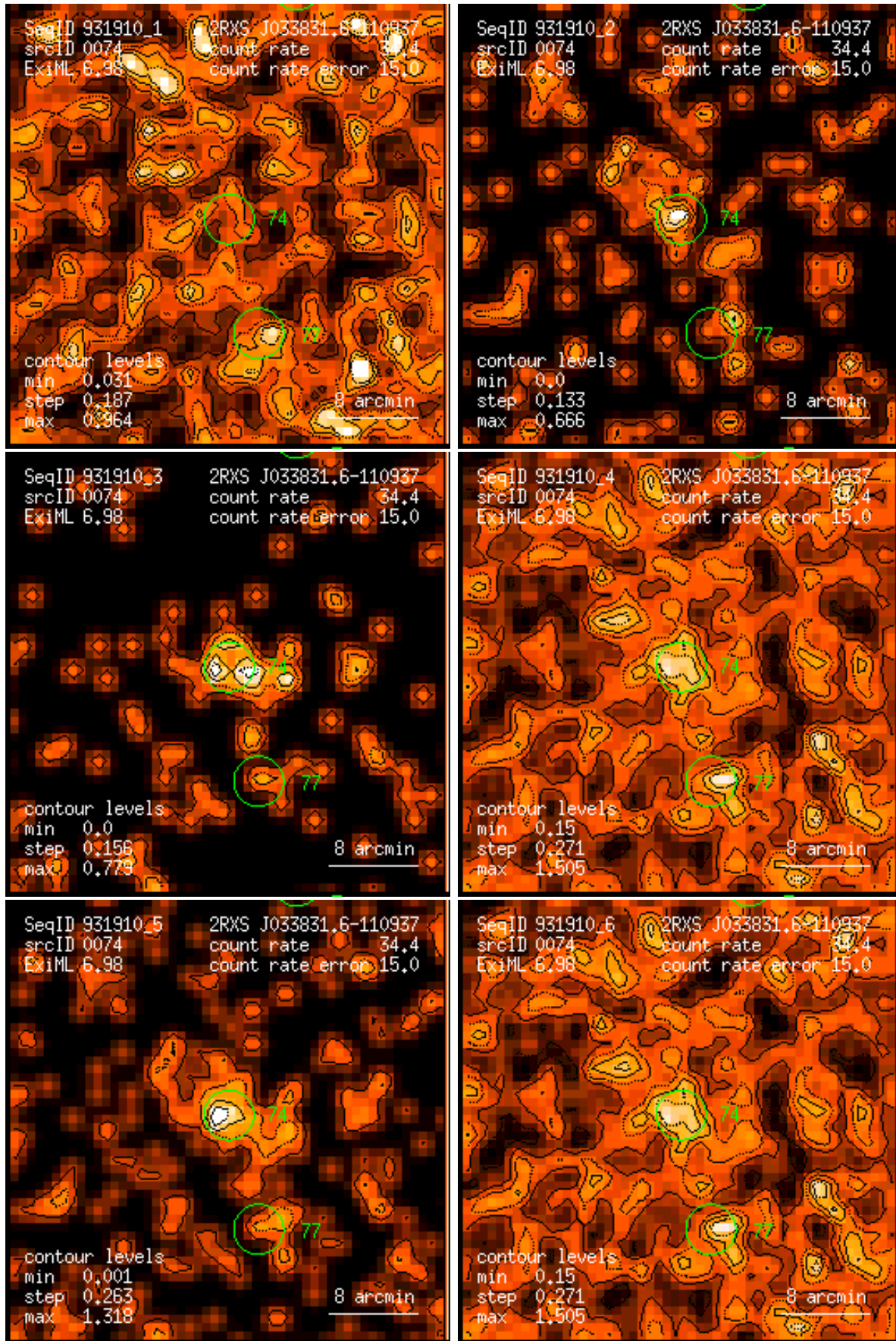
Figure 74: RASS 931910: detection 0074: band rate images, Gaussian filter: (1) PSPC channels 11 – 41, (2) 52 – 90, (3) 91 – 201, (4) 11 – 235, (5) 52 – 201, (6) 11 – 201. Broad band rates in counts/ks. Band rate contour levels in counts/ks/arcmin 2 .
