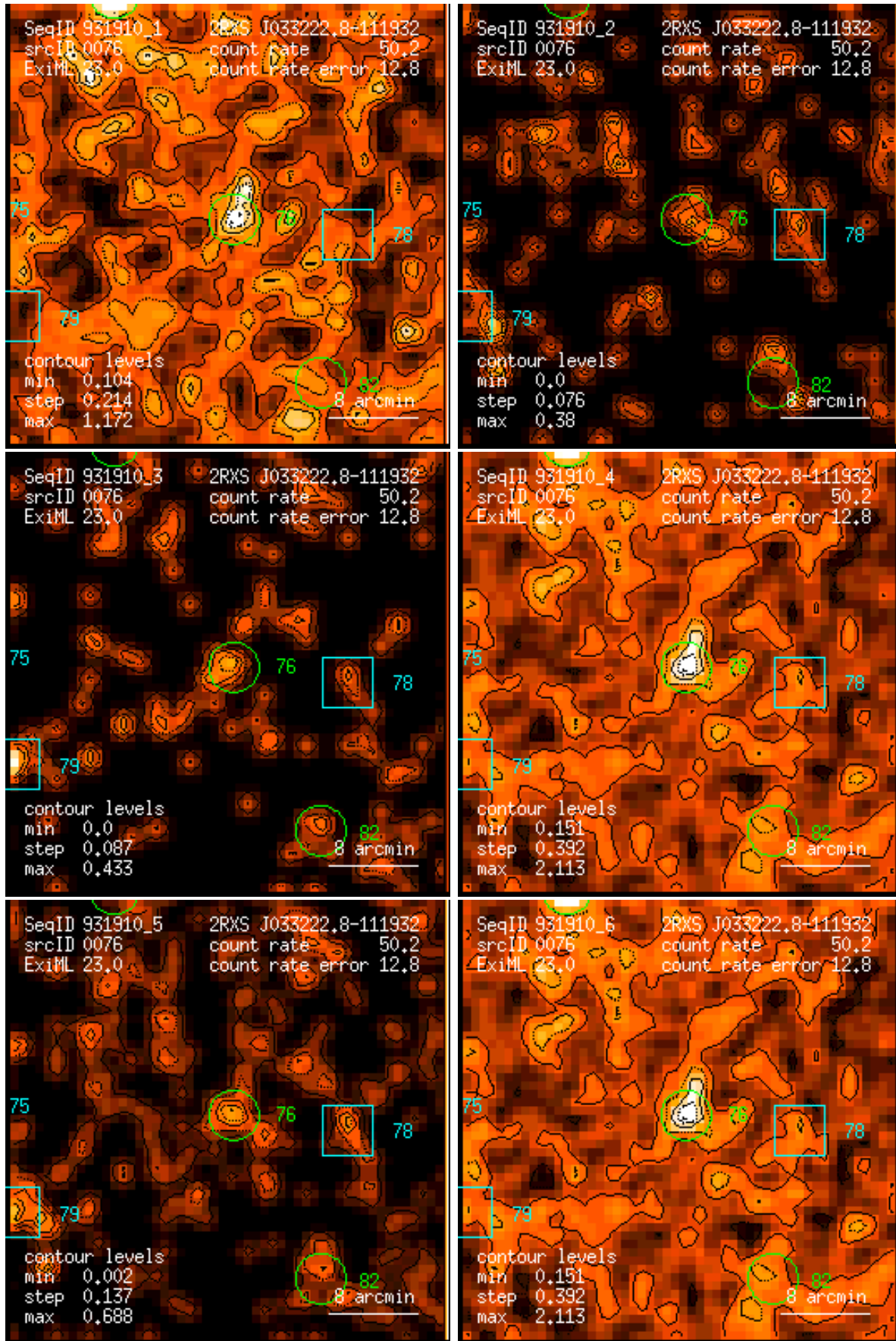
Figure 76: RASS 931910: detection 0076: band rate images, Gaussian filter: (1) PSPC channels 11 – 41, (2) 52 – 90, (3) 91 – 201, (4) 11 – 235, (5) 52 – 201, (6) 11 – 201. Broad band rates in counts/ks. Band rate contour levels in counts/ks/arcmin 2 .
