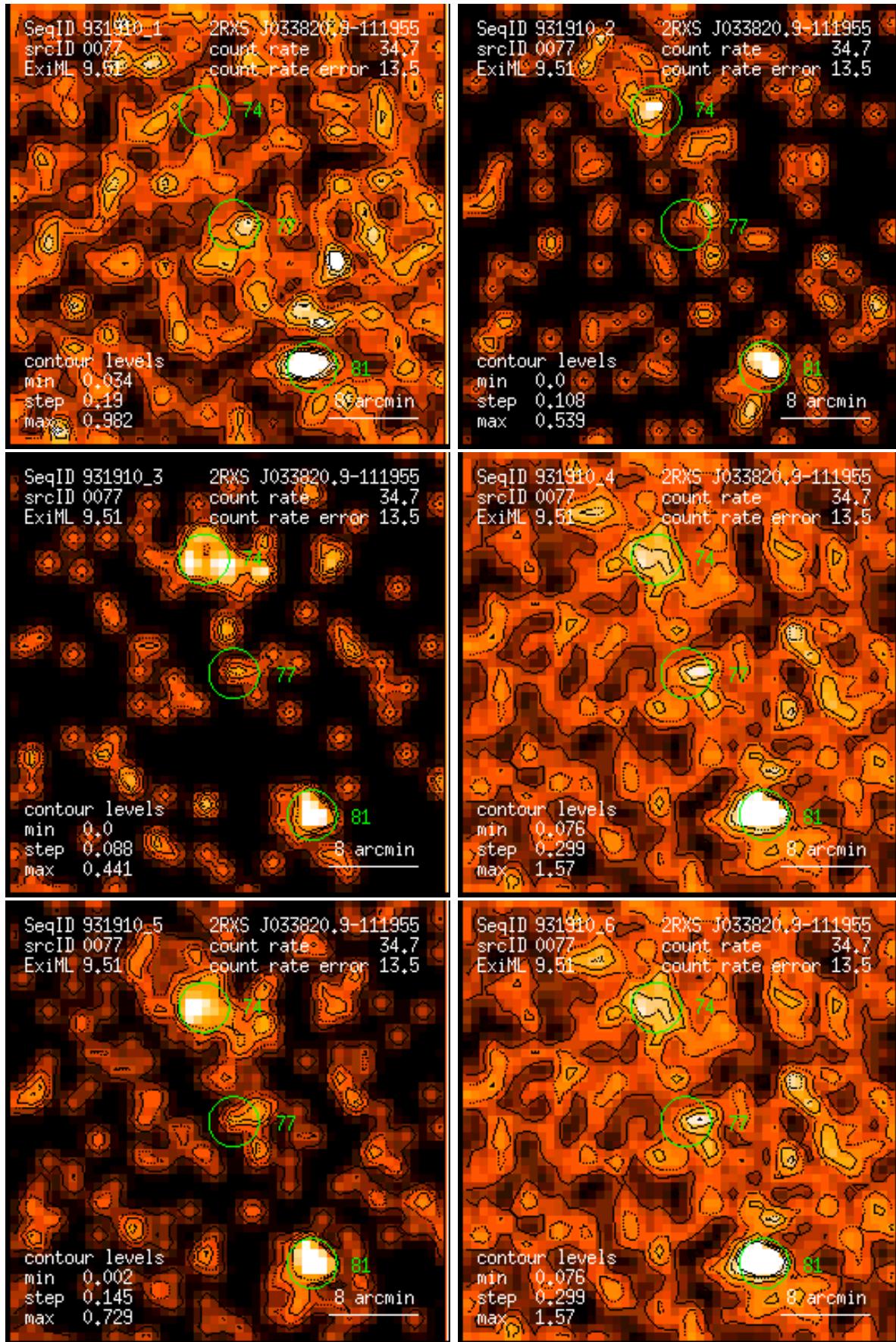
Figure 77: RASS 931910: detection 0077: band rate images, Gaussian filter: (1) PSPC channels 11 – 41, (2) 52 – 90, (3) 91 – 201, (4) 11 – 235, (5) 52 – 201, (6) 11 – 201. Broad band rates in counts/ks. Band rate contour levels in counts/ks/arcmin 2 .
