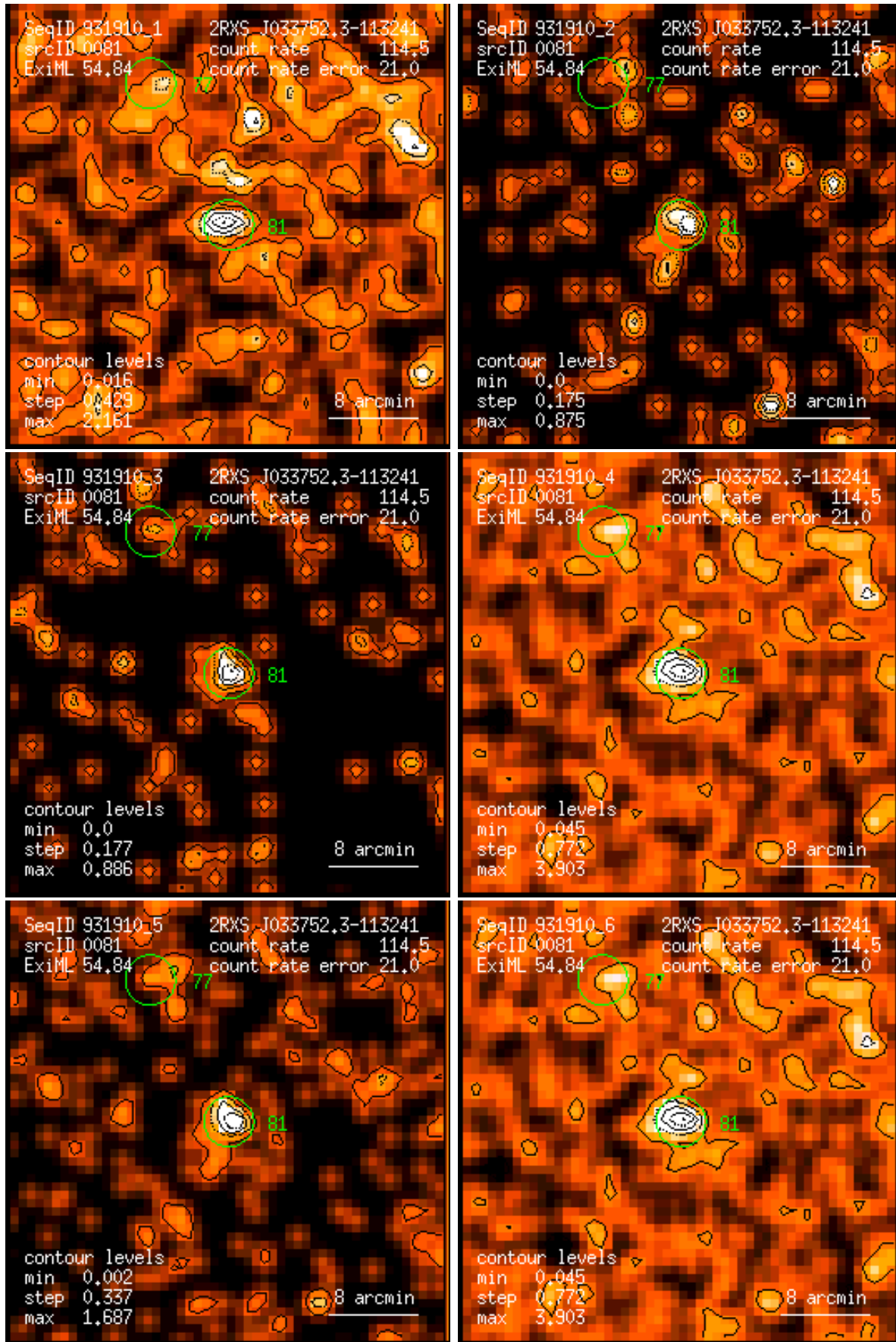
Figure 81: RASS 931910: detection 0081: band rate images, Gaussian filter: (1) PSPC channels 11 – 41, (2) 52 – 90, (3) 91 – 201, (4) 11 – 235, (5) 52 – 201, (6) 11 – 201. Broad band rates in counts/ks. Band rate contour levels in counts/ks/arcmin 2 .
