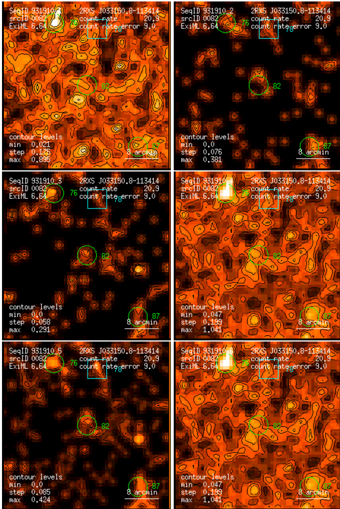
Figure 82: RASS 931910: detection 0082: band rate images, Gaussian filter: (1) PSPC channels 11 – 41, (2) 52 – 90, (3) 91 – 201, (4) 11 – 235, (5) 52 – 201, (6) 11 – 201. Broad band rates in counts/ks. Band rate contour levels in counts/ks/arcmin 2 .
