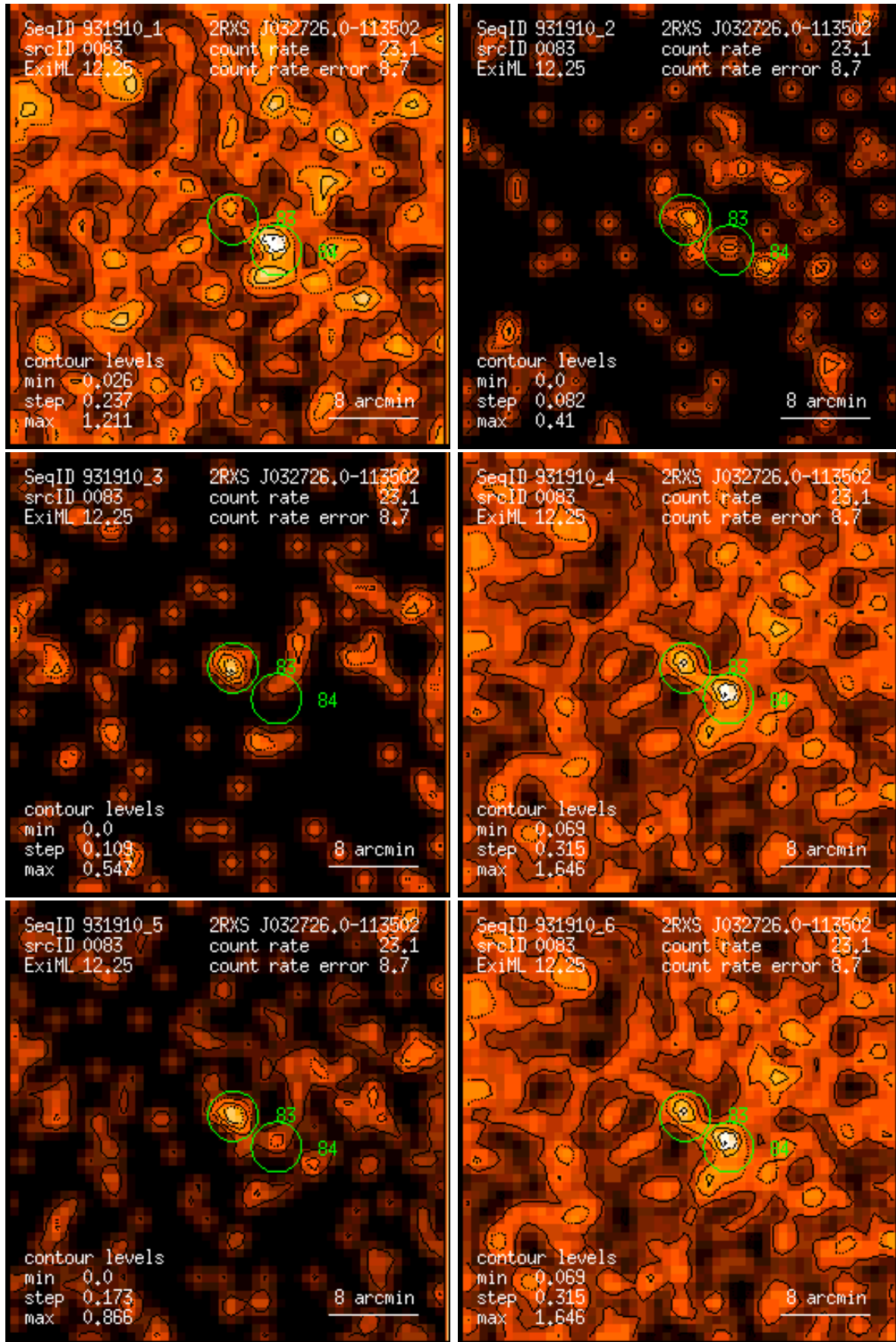
Figure 83: RASS 931910: detection 0083: band rate images, Gaussian filter: (1) PSPC channels 11 – 41, (2) 52 – 90, (3) 91 – 201, (4) 11 – 235, (5) 52 – 201, (6) 11 – 201. Broad band rates in counts/ks. Band rate contour levels in counts/ks/arcmin 2 .
