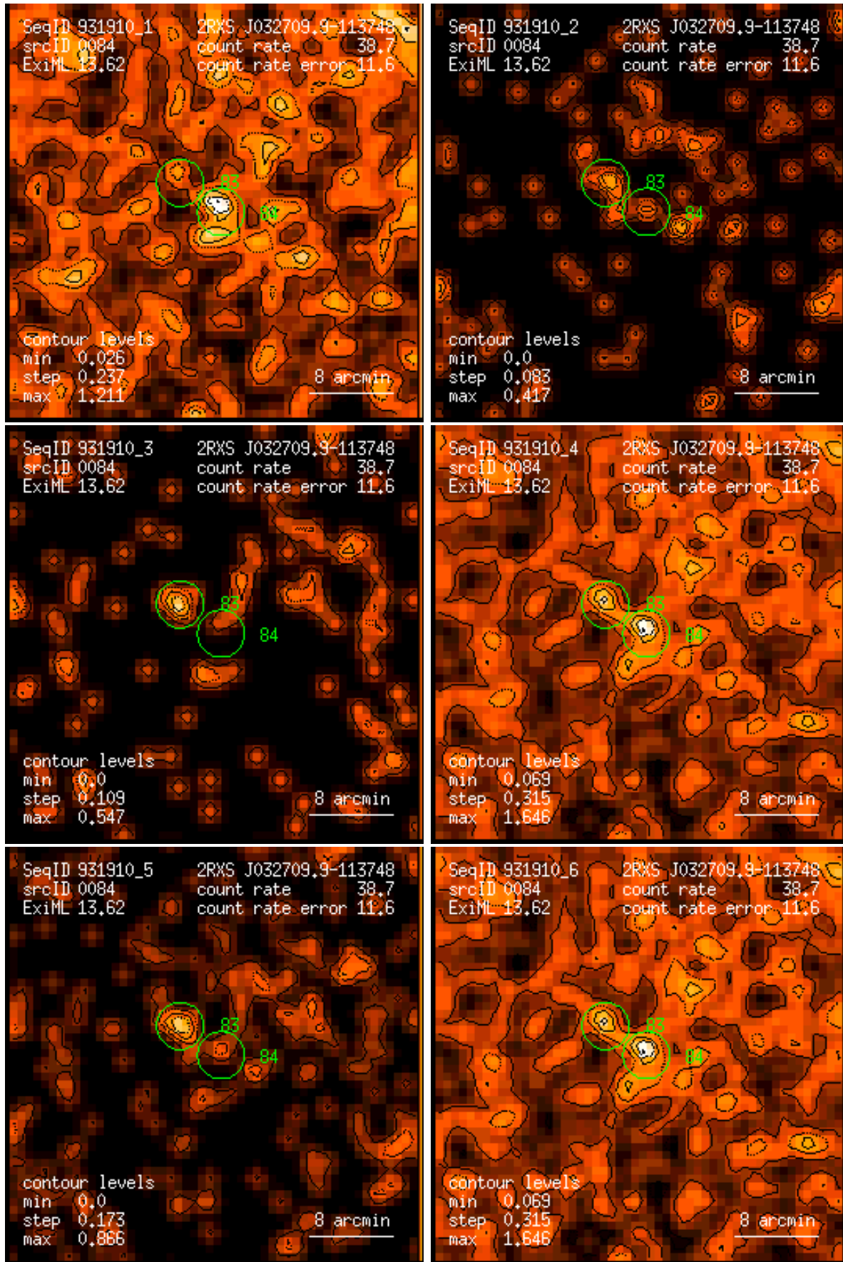
Figure 84: RASS 931910: detection 0084: band rate images, Gaussian filter: (1) PSPC channels 11 – 41, (2) 52 – 90, (3) 91 – 201, (4) 11 – 235, (5) 52 – 201, (6) 11 – 201. Broad band rates in counts/ks. Band rate contour levels in counts/ks/arcmin 2 .
