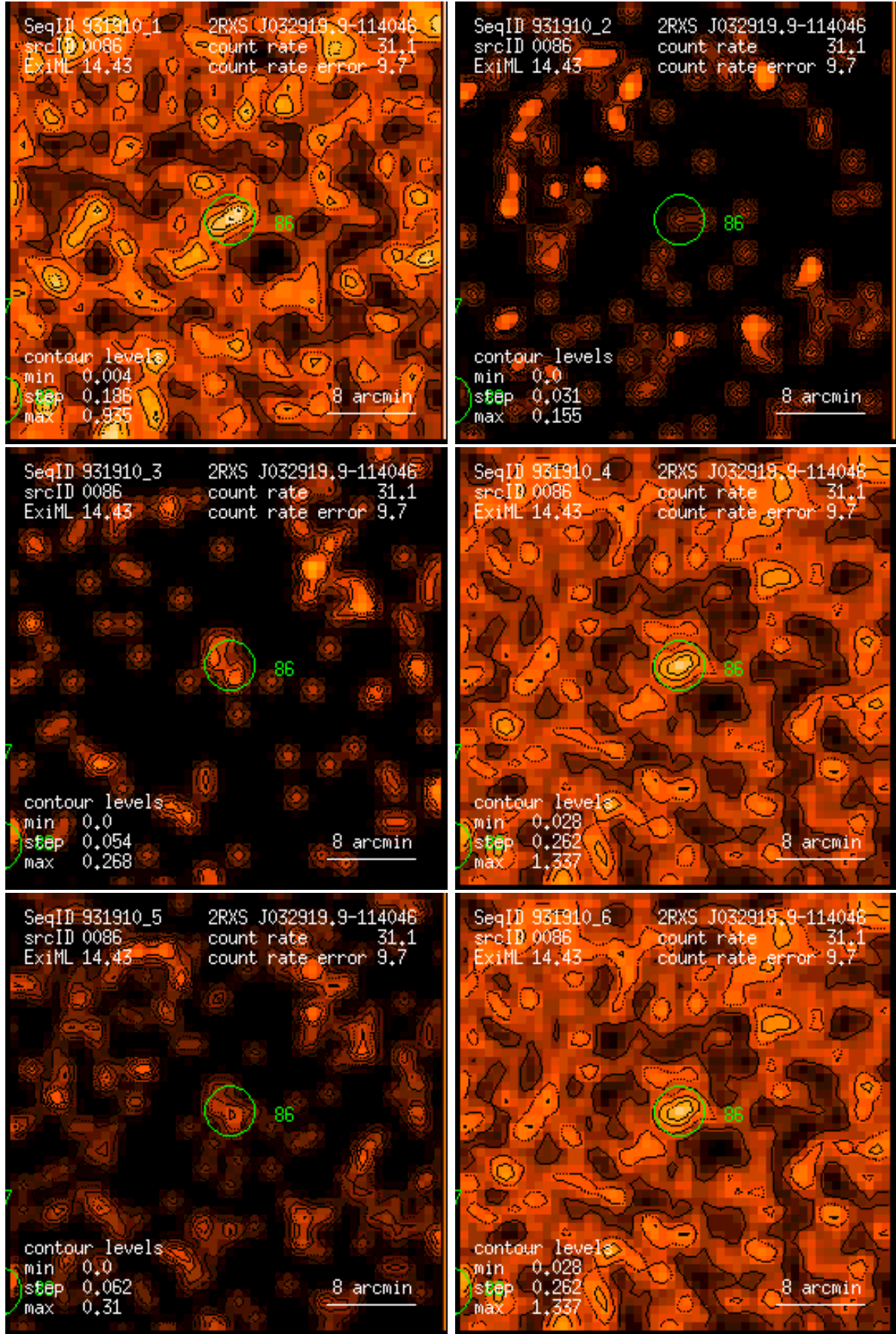
Figure 86: RASS 931910: detection 0086: band rate images, Gaussian filter: (1) PSPC channels 11 – 41, (2) 52 – 90, (3) 91 – 201, (4) 11 – 235, (5) 52 – 201, (6) 11 – 201. Broad band rates in counts/ks. Band rate contour levels in counts/ks/arcmin 2 .
