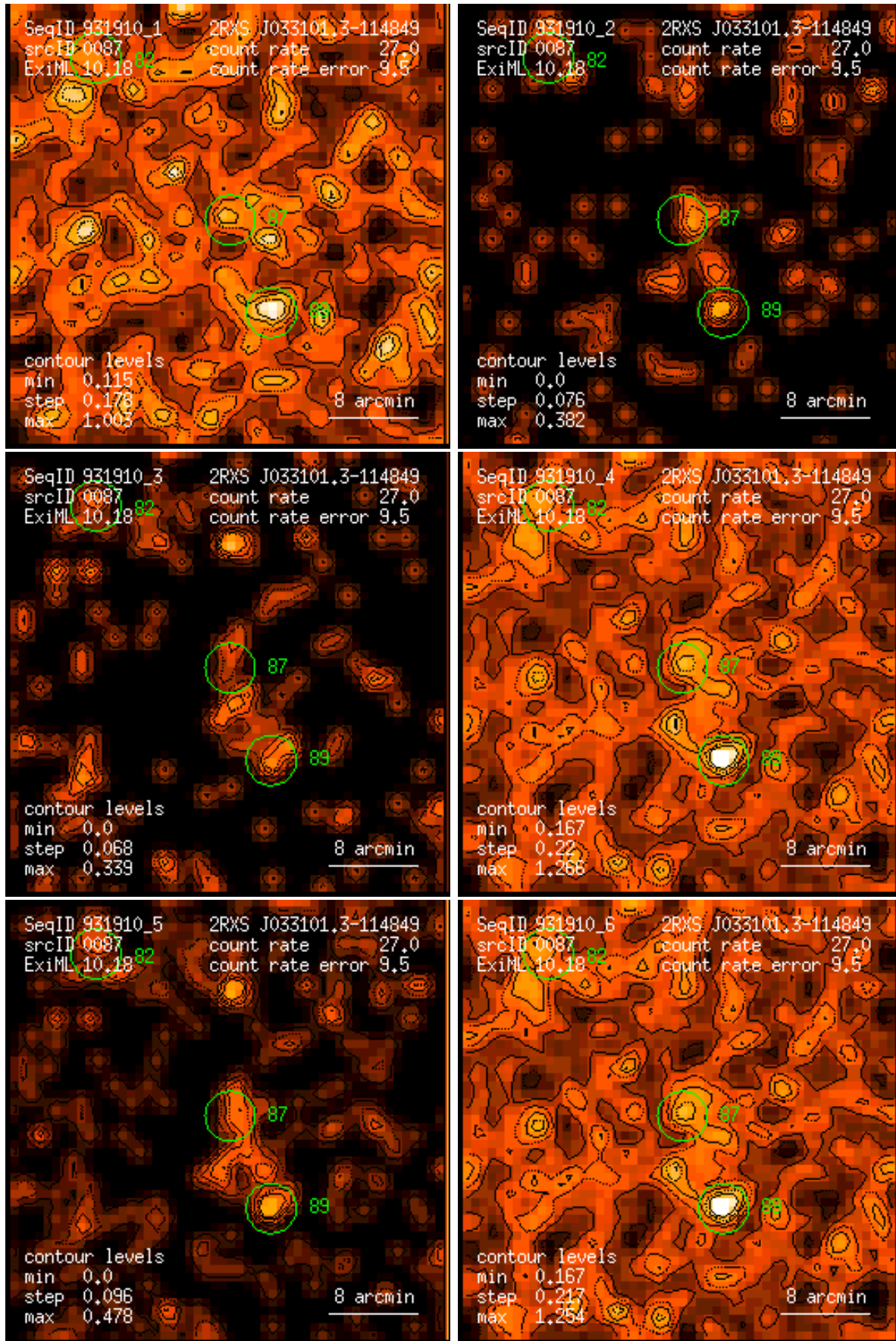
Figure 87: RASS 931910: detection 0087: band rate images, Gaussian filter: (1) PSPC channels 11 – 41, (2) 52 – 90, (3) 91 – 201, (4) 11 – 235, (5) 52 – 201, (6) 11 – 201. Broad band rates in counts/ks. Band rate contour levels in counts/ks/arcmin 2 .
