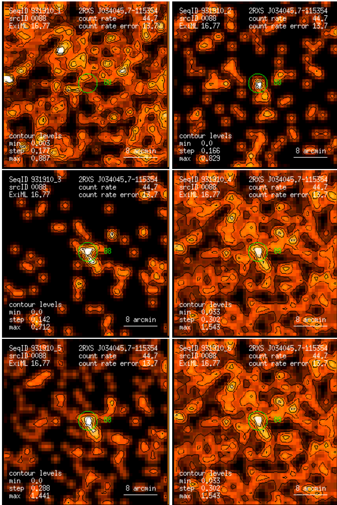
Figure 88: RASS 931910: detection 0088: band rate images, Gaussian filter: (1) PSPC channels 11 – 41, (2) 52 – 90, (3) 91 – 201, (4) 11 – 235, (5) 52 – 201, (6) 11 – 201. Broad band rates in counts/ks. Band rate contour levels in counts/ks/arcmin 2 .
