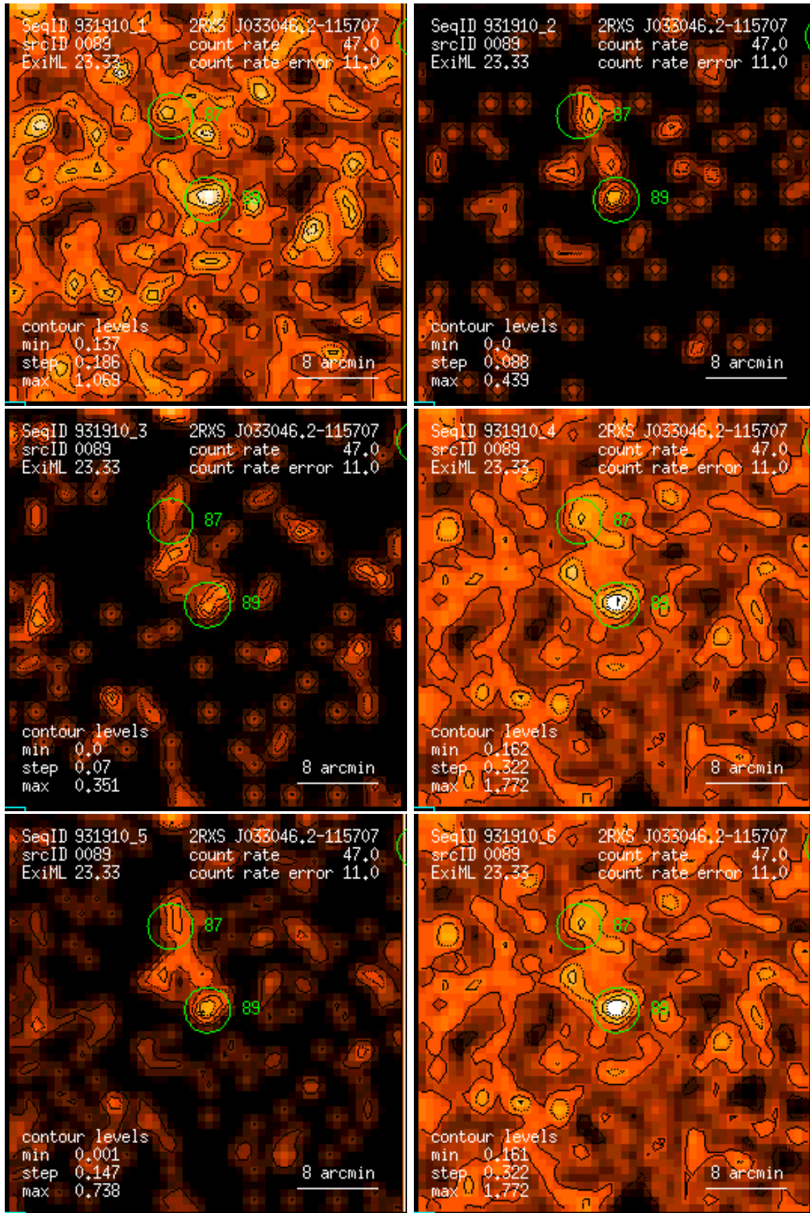
Figure 89: RASS 931910: detection 0089: band rate images, Gaussian filter: (1) PSPC channels 11 – 41, (2) 52 – 90, (3) 91 – 201, (4) 11 – 235, (5) 52 – 201, (6) 11 – 201. Broad band rates in counts/ks. Band rate contour levels in counts/ks/arcmin 2 .
