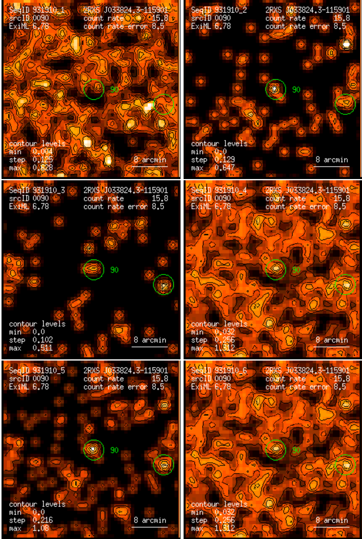
Figure 90: RASS 931910: detection 0090: band rate images, Gaussian filter: (1) PSPC channels 11 – 41, (2) 52 – 90, (3) 91 – 201, (4) 11 – 235, (5) 52 – 201, (6) 11 – 201. Broad band rates in counts/ks. Band rate contour levels in counts/ks/arcmin 2 .
