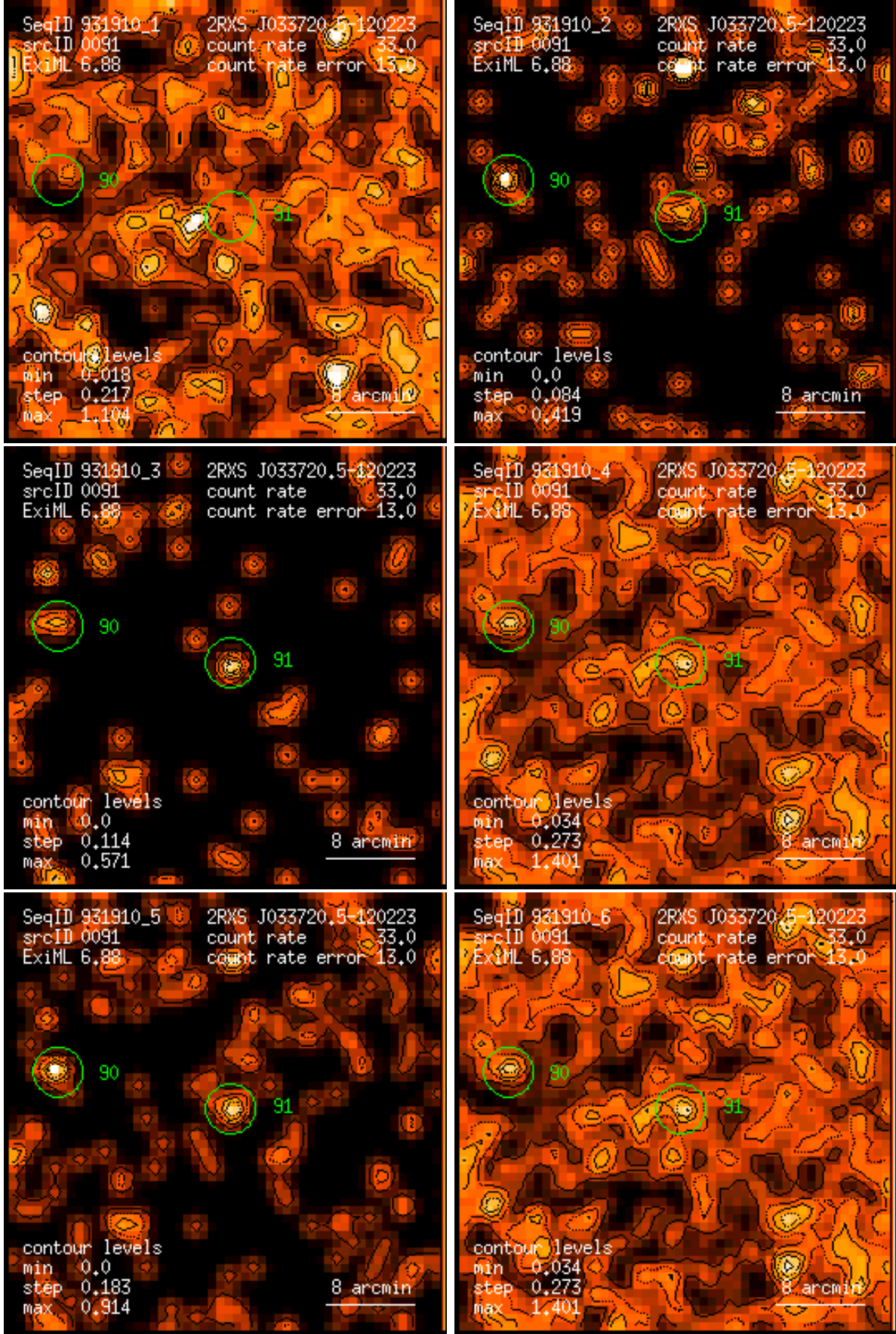
Figure 91: RASS 931910: detection 0091: band rate images, Gaussian filter: (1) PSPC channels 11 – 41, (2) 52 – 90, (3) 91 – 201, (4) 11 – 235, (5) 52 – 201, (6) 11 – 201. Broad band rates in counts/ks. Band rate contour levels in counts/ks/arcmin 2 .
