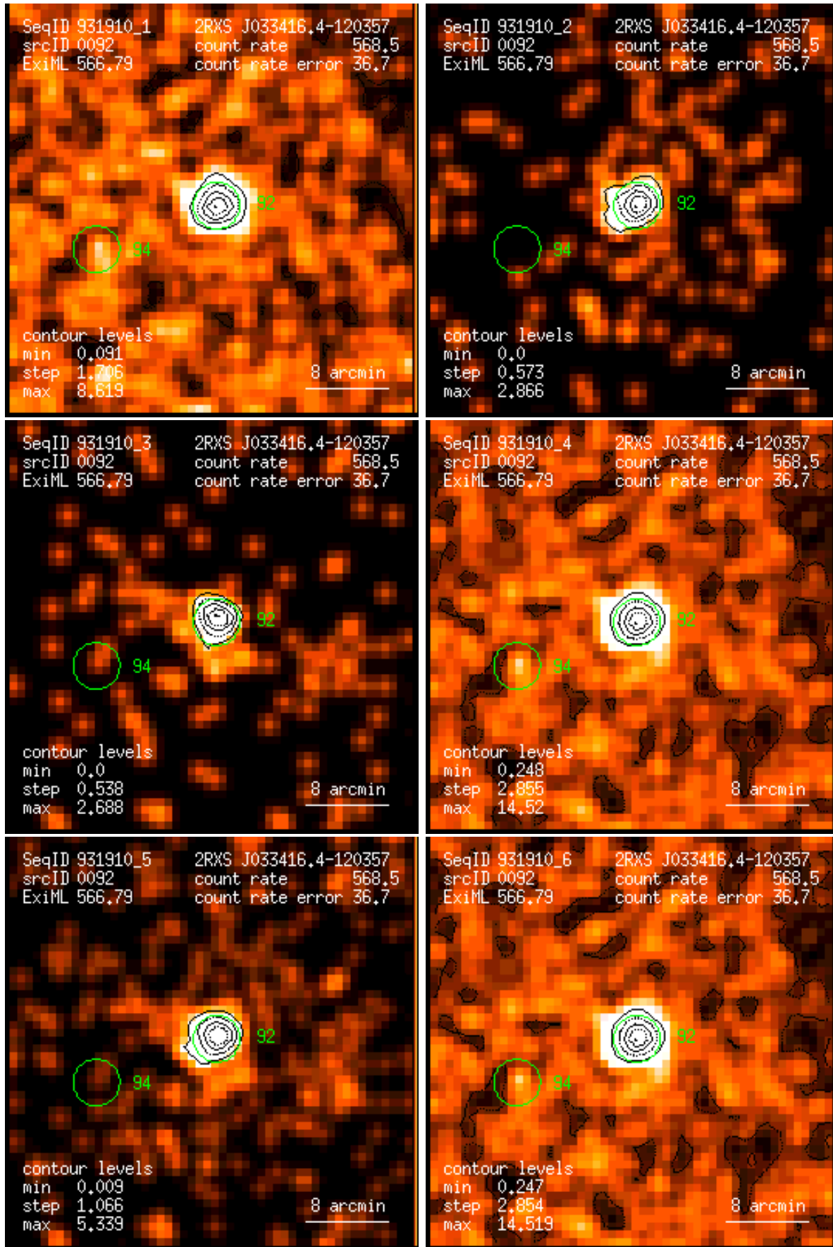
Figure 92: RASS 931910: detection 0092: band rate images, Gaussian filter: (1) PSPC channels 11 – 41, (2) 52 – 90, (3) 91 – 201, (4) 11 – 235, (5) 52 – 201, (6) 11 – 201. Broad band rates in counts/ks. Band rate contour levels in counts/ks/arcmin 2 .
