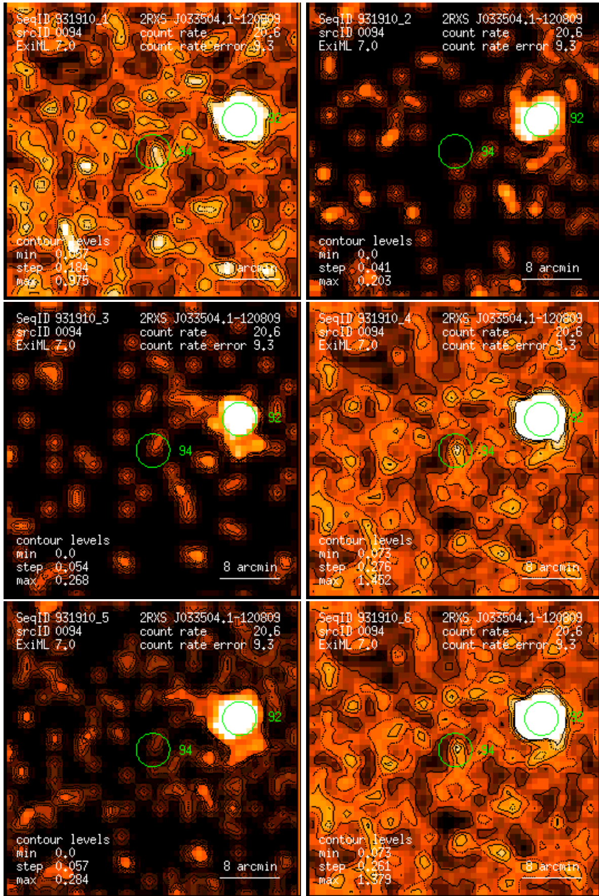
Figure 94: RASS 931910: detection 0094: band rate images, Gaussian filter: (1) PSPC channels 11 – 41, (2) 52 – 90, (3) 91 – 201, (4) 11 – 235, (5) 52 – 201, (6) 11 – 201. Broad band rates in counts/ks. Band rate contour levels in counts/ks/arcmin 2 .
