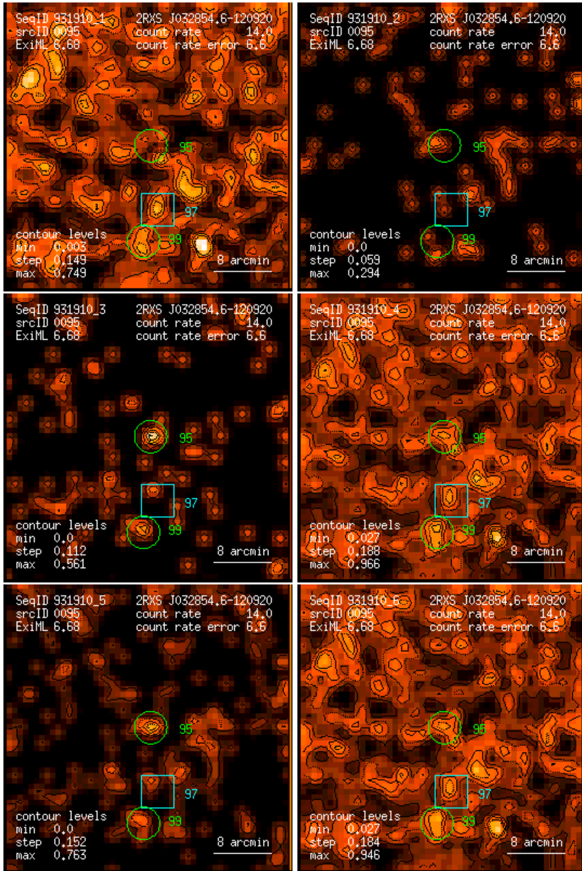
Figure 95: RASS 931910: detection 0095: band rate images, Gaussian filter: (1) PSPC channels 11 – 41, (2) 52 – 90, (3) 91 – 201, (4) 11 – 235, (5) 52 – 201, (6) 11 – 201. Broad band rates in counts/ks. Band rate contour levels in counts/ks/arcmin 2 .
