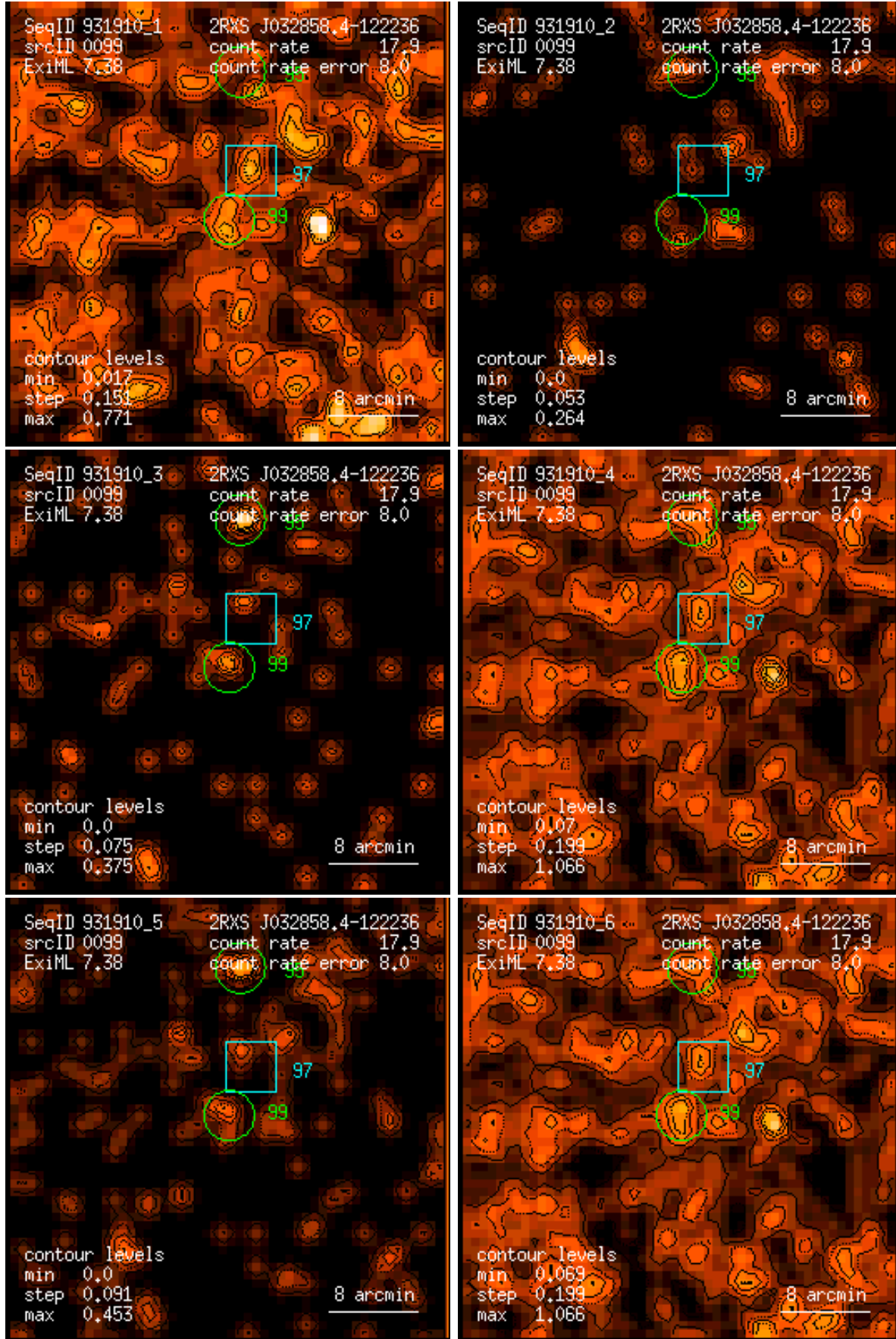
Figure 99: RASS 931910: detection 0099: band rate images, Gaussian filter: (1) PSPC channels 11 – 41, (2) 52 – 90, (3) 91 – 201, (4) 11 – 235, (5) 52 – 201, (6) 11 – 201. Broad band rates in counts/ks. Band rate contour levels in counts/ks/arcmin 2 .
