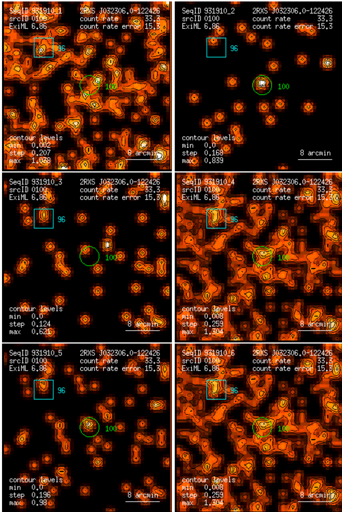
Figure 100: RASS 931910: detection 0100: band rate images, Gaussian filter: (1) PSPC channels 11 – 41, (2) 52 – 90, (3) 91 – 201, (4) 11 – 235, (5) 52 – 201, (6) 11 – 201. Broad band rates in counts/ks. Band rate contour levels in counts/ks/arcmin 2 .
