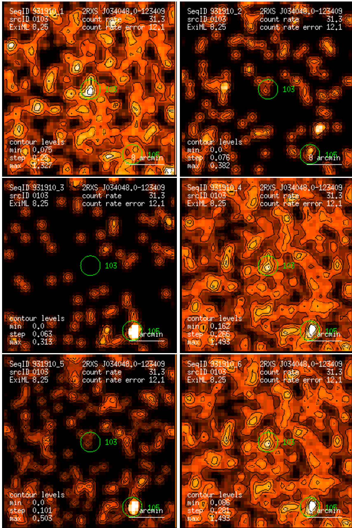
Figure 103: RASS 931910: detection 0103: band rate images, Gaussian filter: (1) PSPC channels 11 – 41, (2) 52 – 90, (3) 91 – 201, (4) 11 – 235, (5) 52 – 201, (6) 11 – 201. Broad band rates in counts/ks. Band rate contour levels in counts/ks/arcmin 2 .
