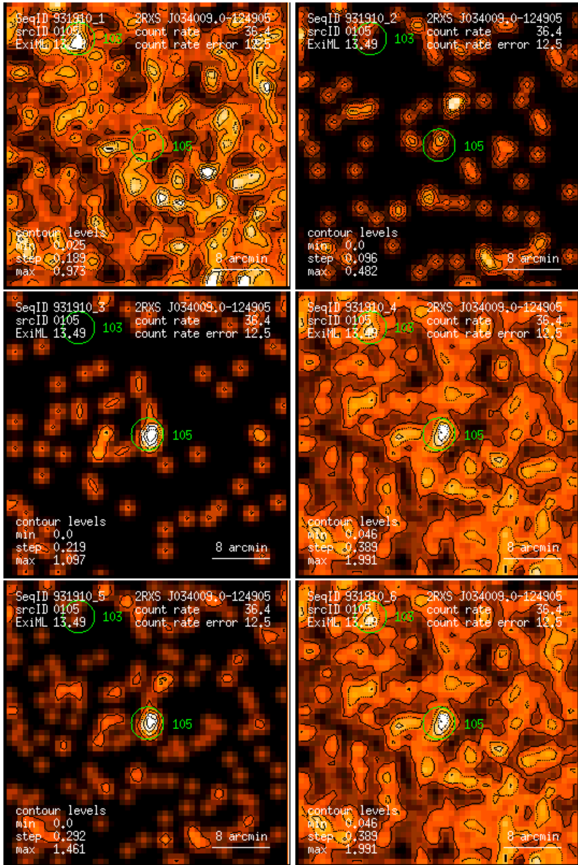
Figure 105: RASS 931910: detection 0105: band rate images, Gaussian filter: (1) PSPC channels 11 – 41, (2) 52 – 90, (3) 91 – 201, (4) 11 – 235, (5) 52 – 201, (6) 11 – 201. Broad band rates in counts/ks. Band rate contour levels in counts/ks/arcmin 2 .
