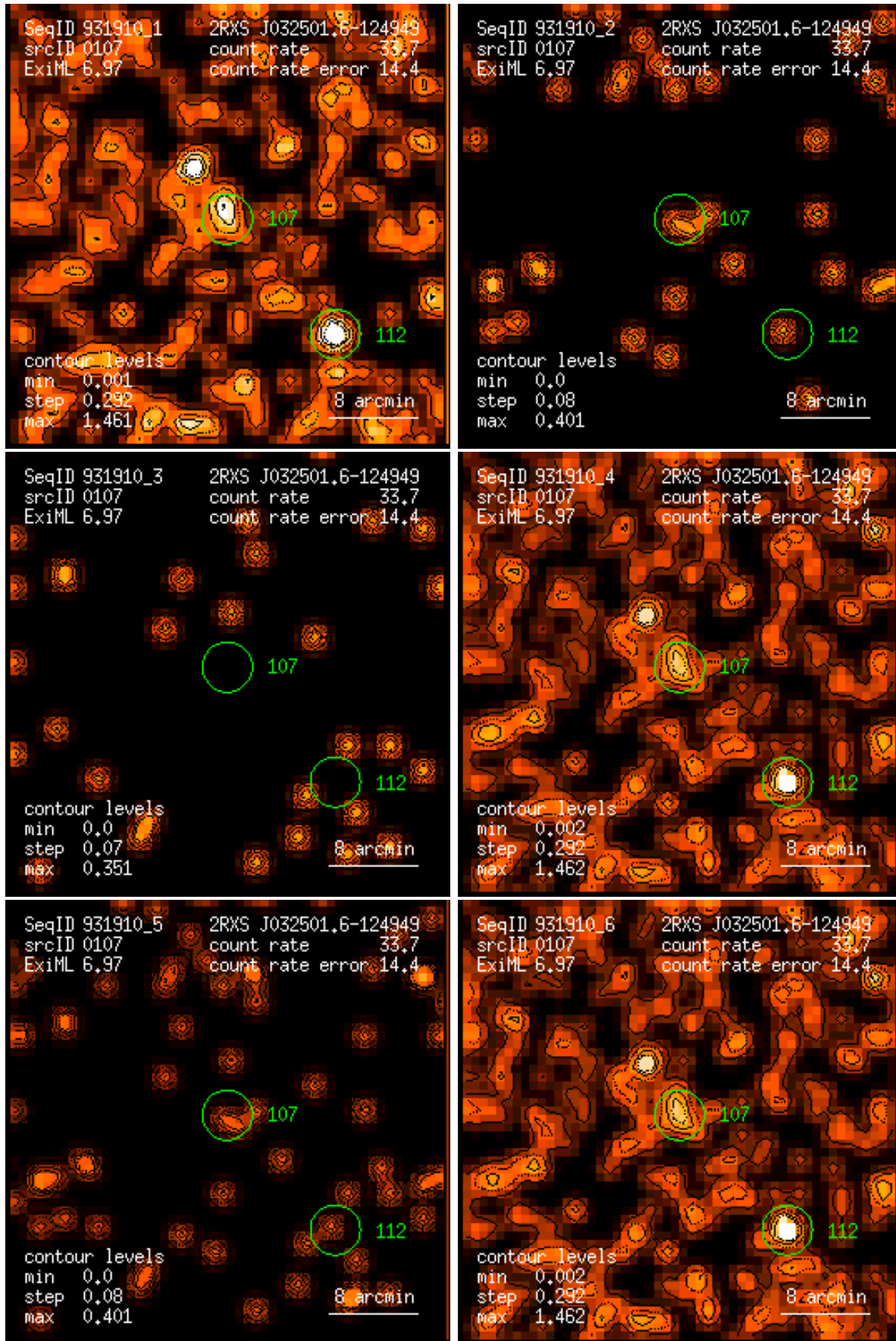
Figure 107: RASS 931910: detection 0107: band rate images, Gaussian filter: (1) PSPC channels 11 – 41, (2) 52 – 90, (3) 91 – 201, (4) 11 – 235, (5) 52 – 201, (6) 11 – 201. Broad band rates in counts/ks. Band rate contour levels in counts/ks/arcmin 2 .
