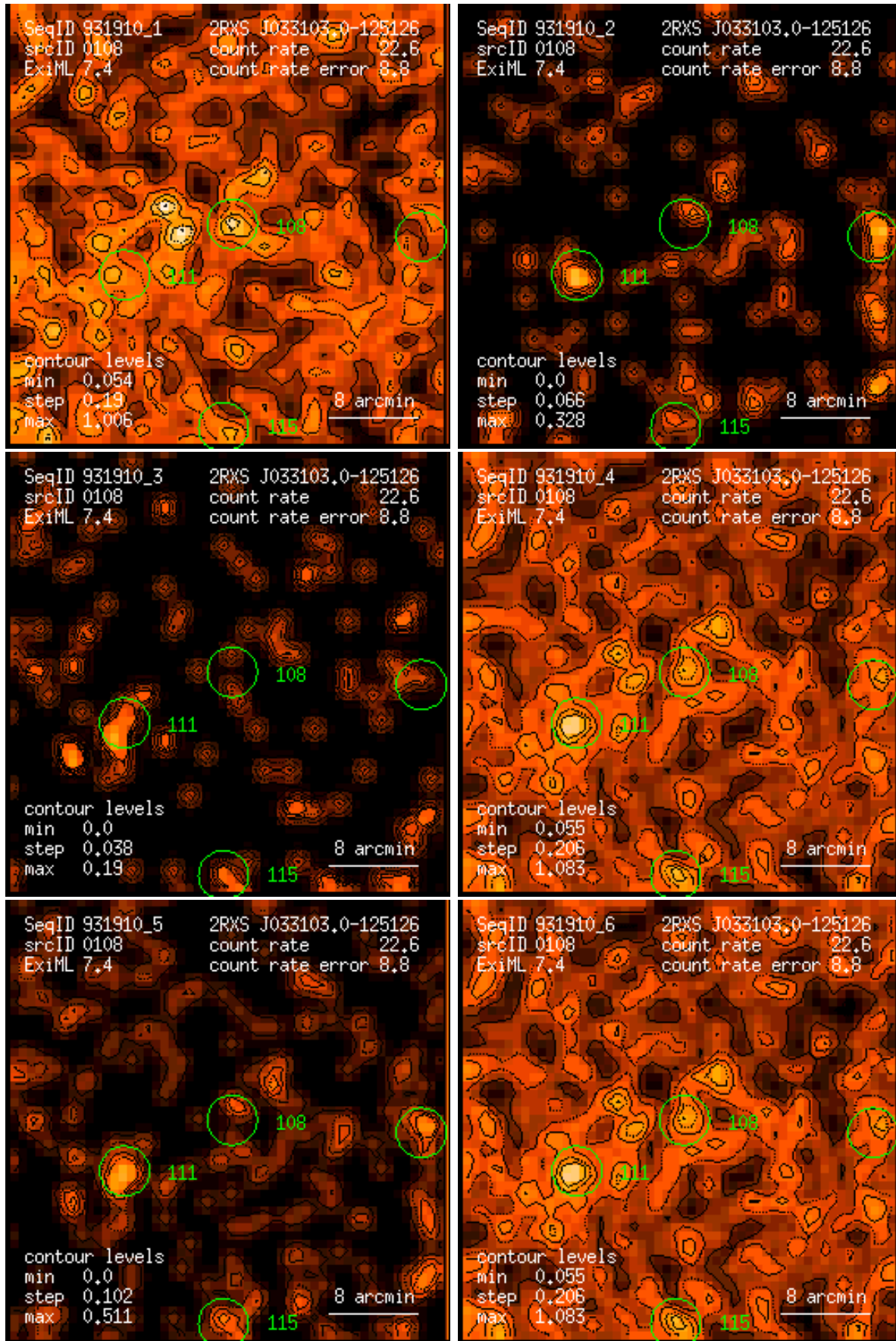
Figure 108: RASS 931910: detection 0108: band rate images, Gaussian filter: (1) PSPC channels 11 – 41, (2) 52 – 90, (3) 91 – 201, (4) 11 – 235, (5) 52 – 201, (6) 11 – 201. Broad band rates in counts/ks. Band rate contour levels in counts/ks/arcmin 2 .
