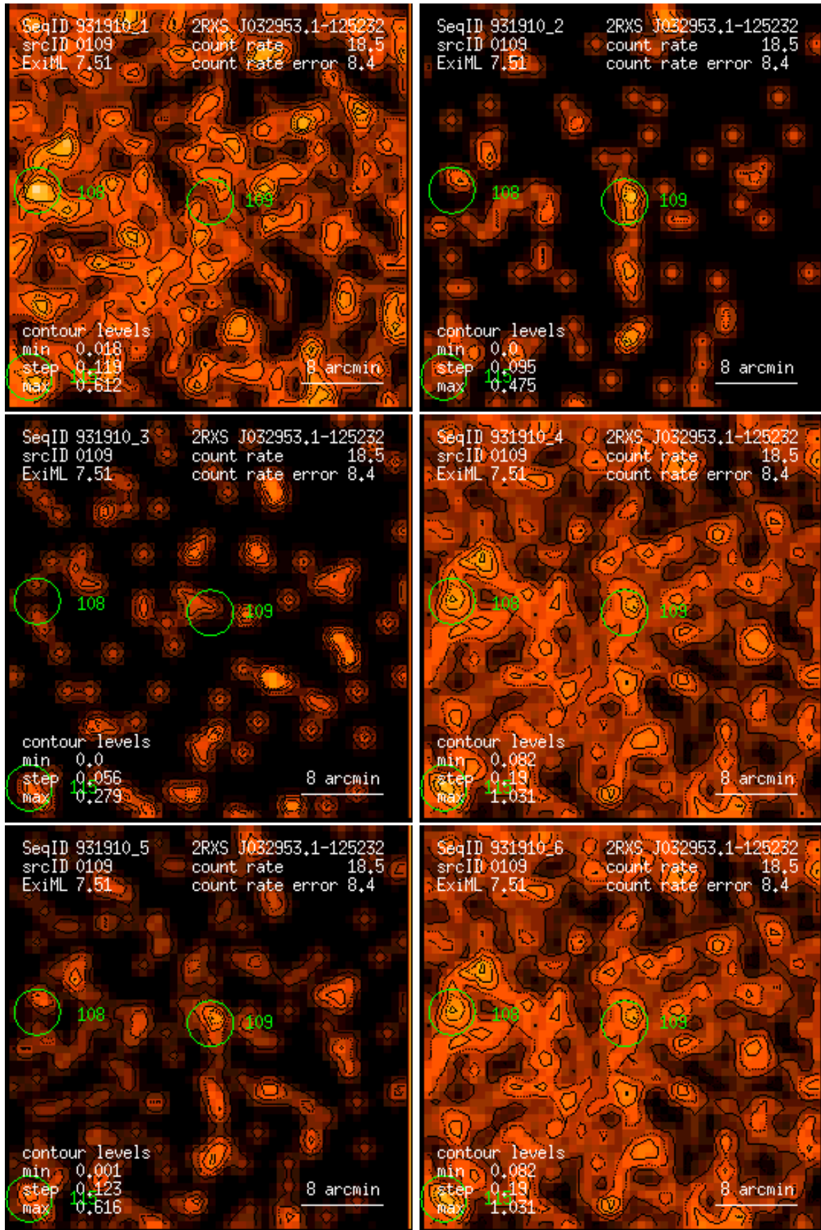
Figure 109: RASS 931910: detection 0109: band rate images, Gaussian filter: (1) PSPC channels 11 – 41, (2) 52 – 90, (3) 91 – 201, (4) 11 – 235, (5) 52 – 201, (6) 11 – 201. Broad band rates in counts/ks. Band rate contour levels in counts/ks/arcmin 2 .
