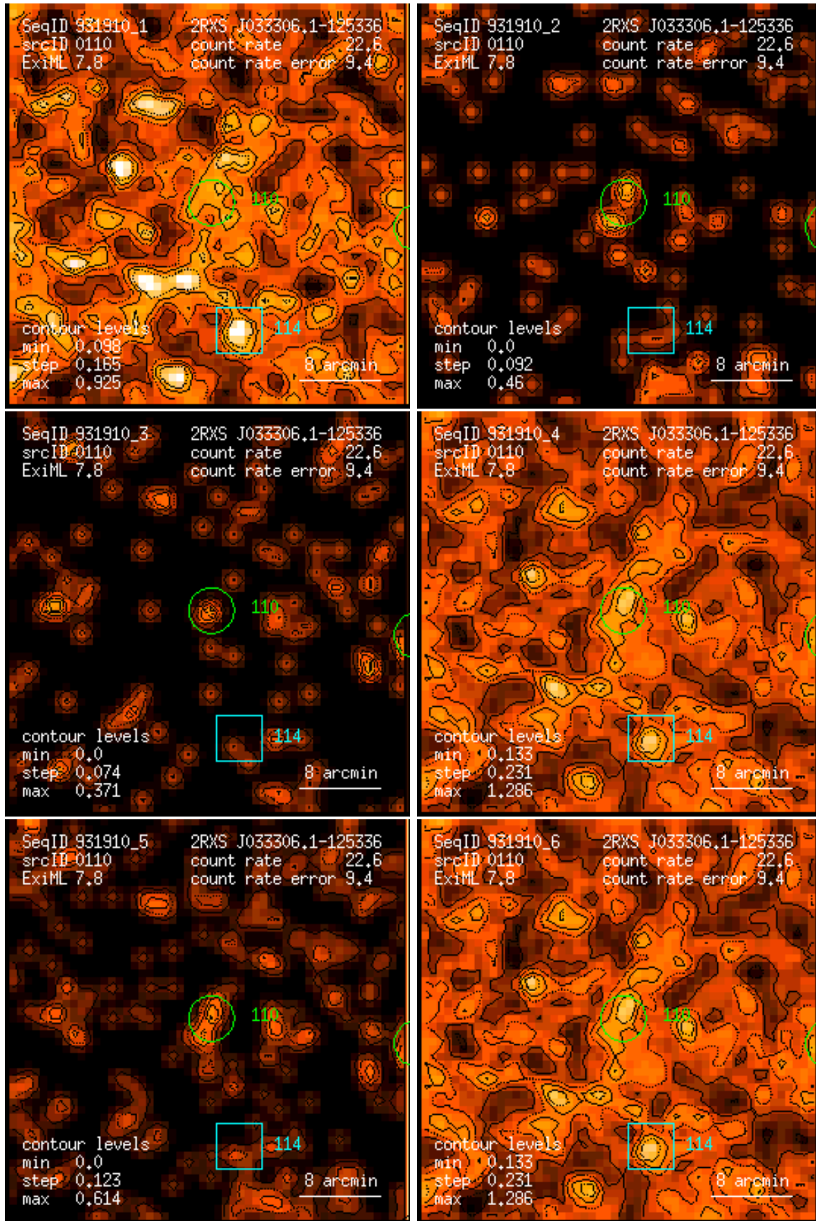
Figure 110: RASS 931910: detection 0110: band rate images, Gaussian filter: (1) PSPC channels 11 – 41, (2) 52 – 90, (3) 91 – 201, (4) 11 – 235, (5) 52 – 201, (6) 11 – 201. Broad band rates in counts/ks. Band rate contour levels in counts/ks/arcmin 2 .
