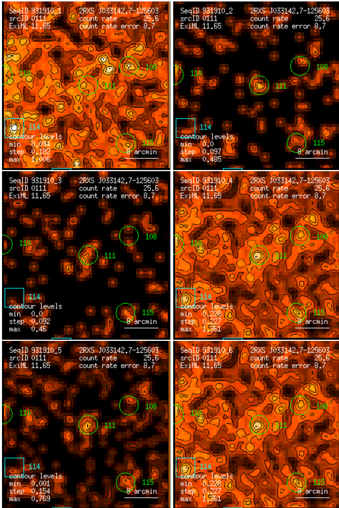
Figure 111: RASS 931910: detection 0111: band rate images, Gaussian filter: (1) PSPC channels 11 – 41, (2) 52 – 90, (3) 91 – 201, (4) 11 – 235, (5) 52 – 201, (6) 11 – 201. Broad band rates in counts/ks. Band rate contour levels in counts/ks/arcmin 2 .
