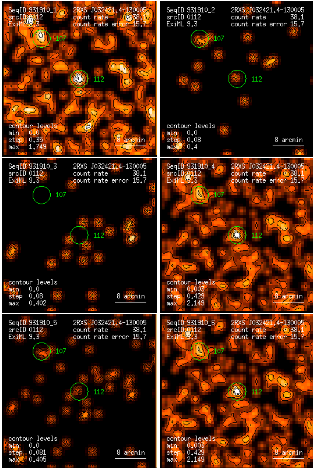
Figure 112: RASS 931910: detection 0112: band rate images, Gaussian filter: (1) PSPC channels 11 – 41, (2) 52 – 90, (3) 91 – 201, (4) 11 – 235, (5) 52 – 201, (6) 11 – 201. Broad band rates in counts/ks. Band rate contour levels in counts/ks/arcmin 2 .
