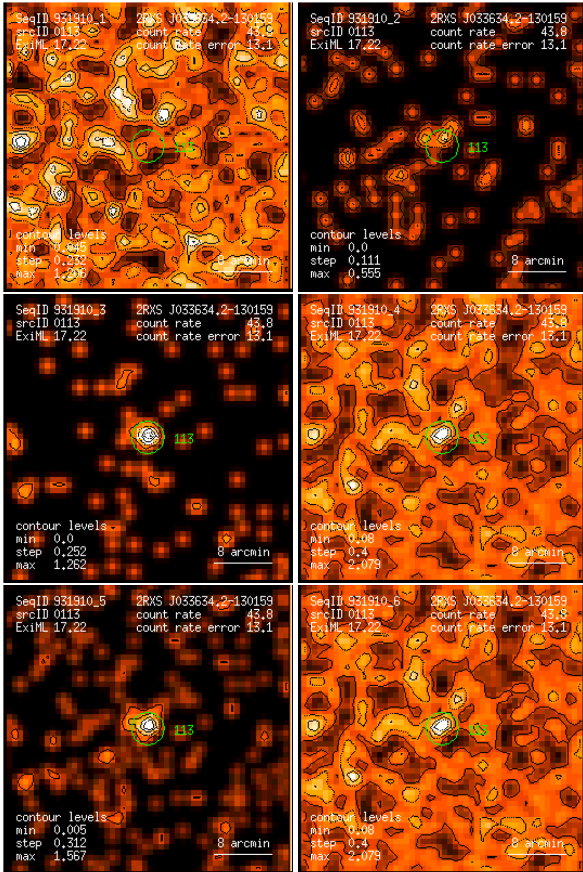
Figure 113: RASS 931910: detection 0113: band rate images, Gaussian filter: (1) PSPC channels 11 – 41, (2) 52 – 90, (3) 91 – 201, (4) 11 – 235, (5) 52 – 201, (6) 11 – 201. Broad band rates in counts/ks. Band rate contour levels in counts/ks/arcmin 2 .
