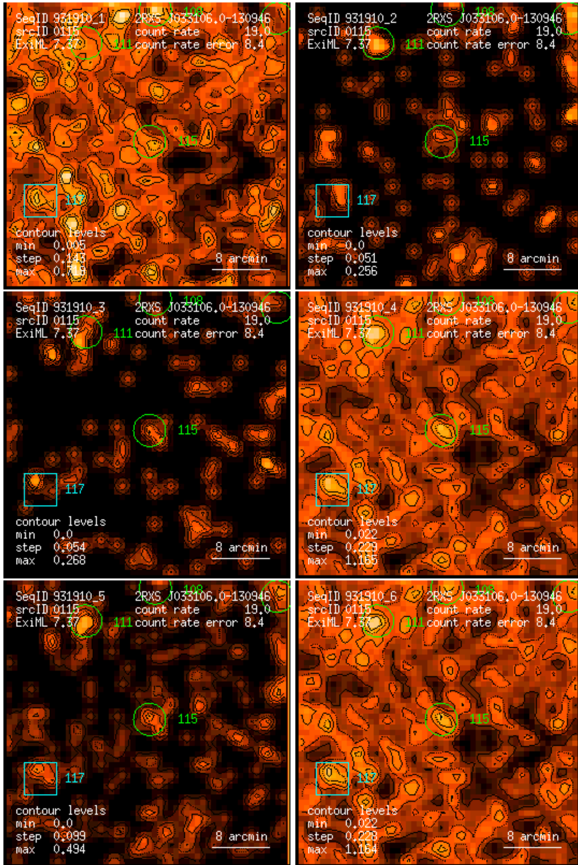
Figure 115: RASS 931910: detection 0115: band rate images, Gaussian filter: (1) PSPC channels 11 – 41, (2) 52 – 90, (3) 91 – 201, (4) 11 – 235, (5) 52 – 201, (6) 11 – 201. Broad band rates in counts/ks. Band rate contour levels in counts/ks/arcmin 2 .
