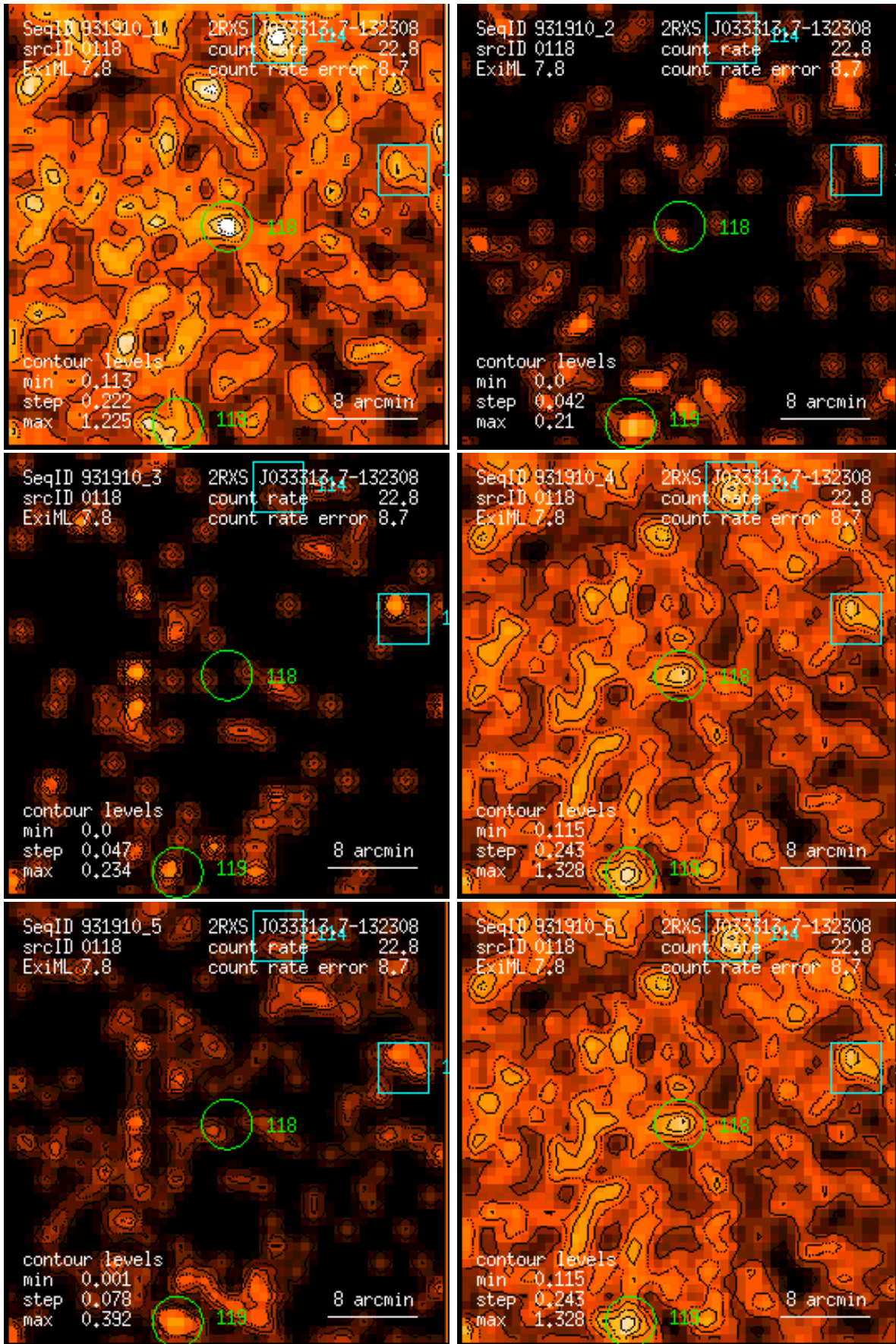
Figure 118: RASS 931910: detection 0118: band rate images, Gaussian filter: (1) PSPC channels 11 – 41, (2) 52 – 90, (3) 91 – 201, (4) 11 – 235, (5) 52 – 201, (6) 11 – 201. Broad band rates in counts/ks. Band rate contour levels in counts/ks/arcmin 2 .
