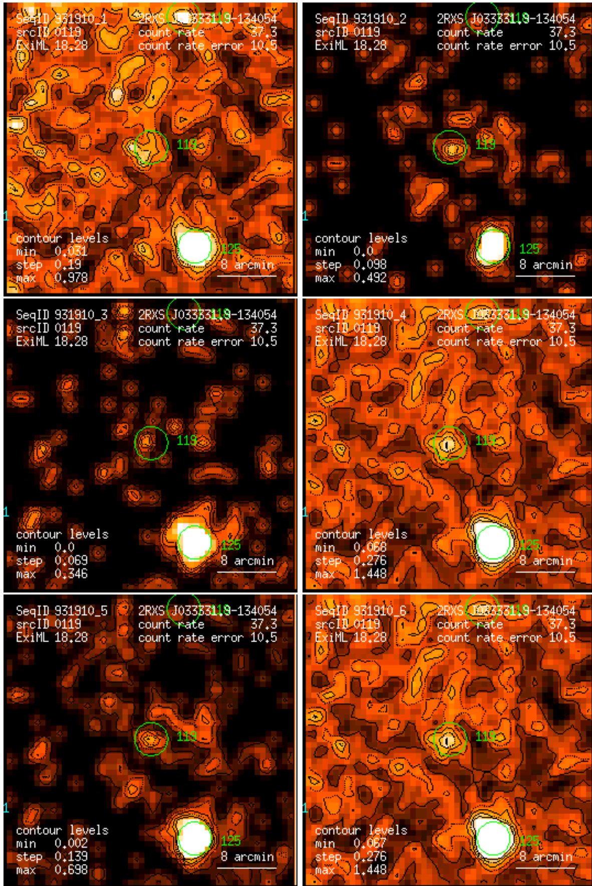
Figure 119: RASS 931910: detection 0119: band rate images, Gaussian filter: (1) PSPC channels 11 – 41, (2) 52 – 90, (3) 91 – 201, (4) 11 – 235, (5) 52 – 201, (6) 11 – 201. Broad band rates in counts/ks. Band rate contour levels in counts/ks/arcmin 2 .
