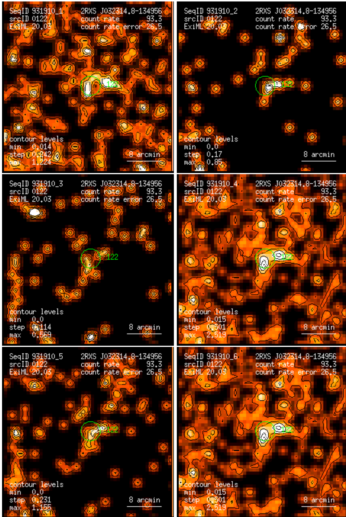
Figure 122: RASS 931910: detection 0122: band rate images, Gaussian filter: (1) PSPC channels 11 – 41, (2) 52 – 90, (3) 91 – 201, (4) 11 – 235, (5) 52 – 201, (6) 11 – 201. Broad band rates in counts/ks. Band rate contour levels in counts/ks/arcmin 2 .
