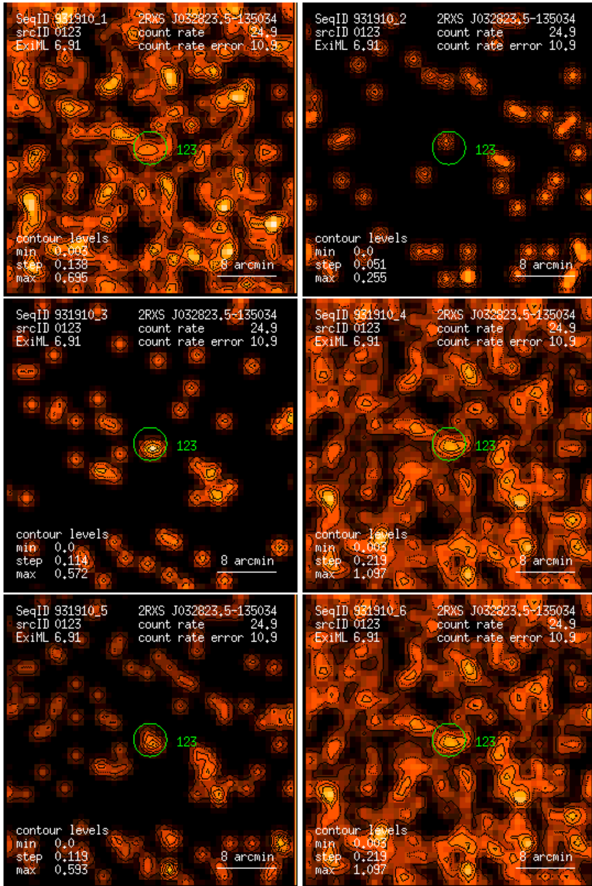
Figure 123: RASS 931910: detection 0123: band rate images, Gaussian filter: (1) PSPC channels 11 – 41, (2) 52 – 90, (3) 91 – 201, (4) 11 – 235, (5) 52 – 201, (6) 11 – 201. Broad band rates in counts/ks. Band rate contour levels in counts/ks/arcmin 2 .
